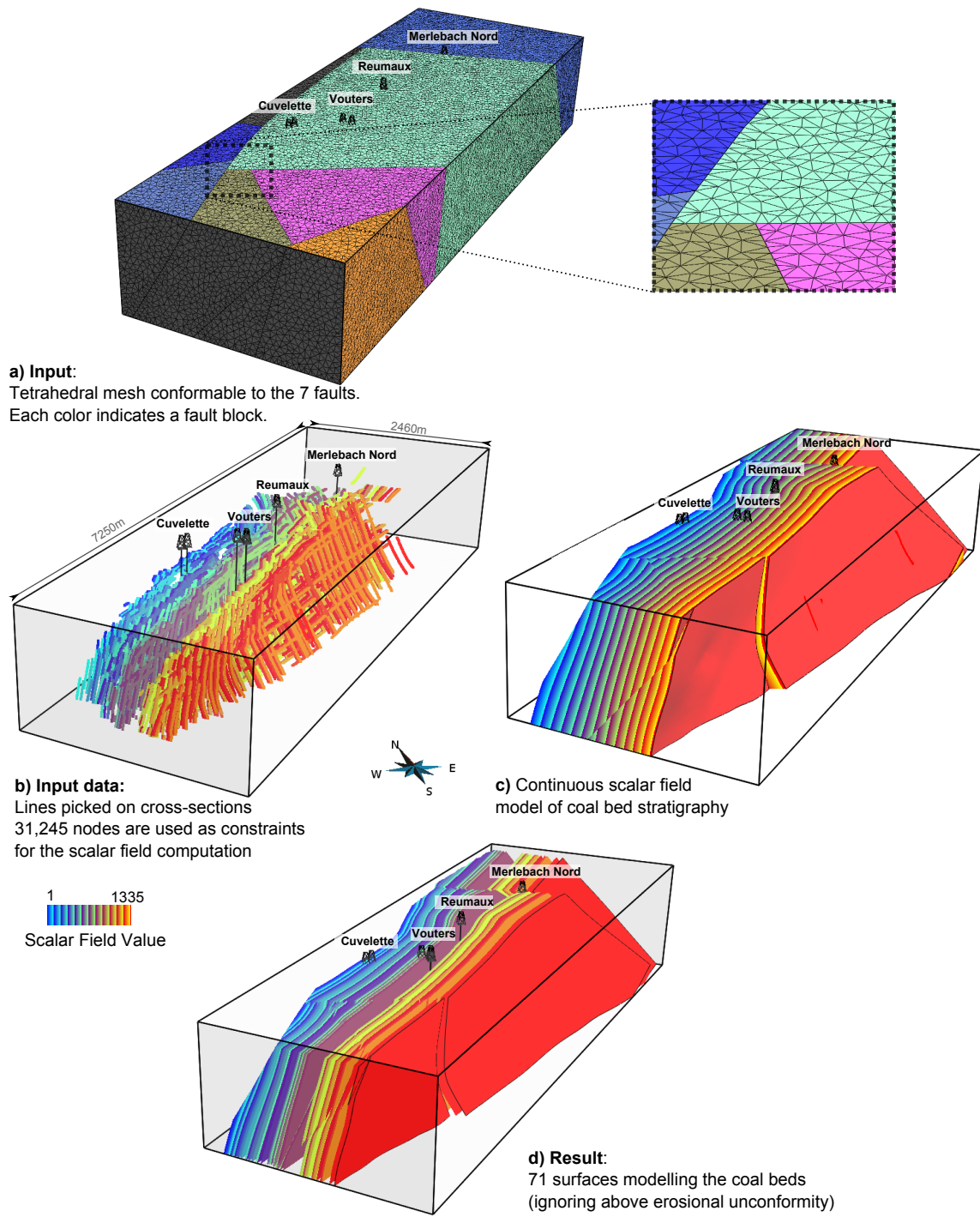
Figure 10: Implicit modelling of the coal beds.
