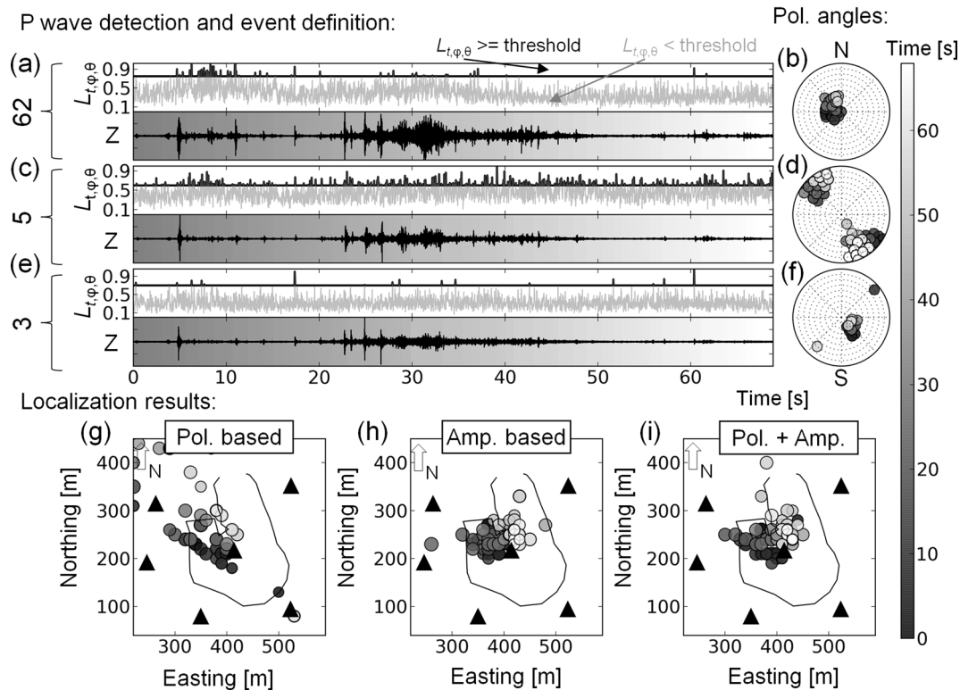
Figure 15. Location results for swarming sequence example 2. Further descriptions are given in Fig. 13. For a better illustration, the minimum expected source origin times \tau_{\text{start}}^i of the identified events are not shown here.
