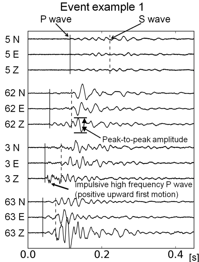
Figure 4. Microseismic wave form example. Unfiltered wave forms for event 1 (Fig. 3) shown for all four three-component stations.
