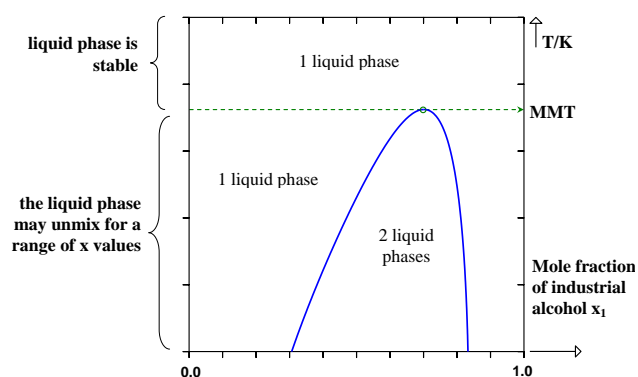
Figure 2. Pseudo-binary phase diagram for a mixture of gasoil and industrial alcohol. The bell is the boundary between the single liquid and the two-liquid fields (saturation curve). MMT is the summit of the saturation curve.
