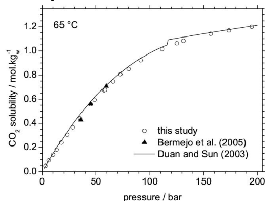
Fig. 5: \text{CO}_2 solubility as a function of pressure at 65 °C calculated from Raman data and fit at 100 °C (Fig. 3). Line: thermodynamic model of Duan and Sun (2003); Void circles: this study (average value, Y-error bar equal or lower to point size); plain triangles: literature data (Bermejo et al., 2005).
