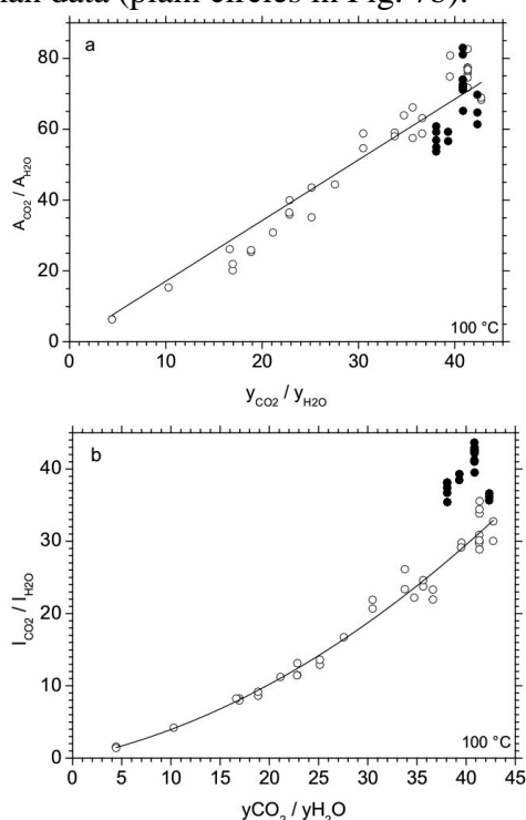
Fig. 7: (a): A_{\text{CO}_2}/A_{\text{H}_2\text{O}} peak area ratio (arbitrary units) as a function of y_{\text{CO}_2}/y_{\text{H}_2\text{O}} molar fraction in vapor phase calculated using the thermodynamic model of Duan and Sun (2003) at 100 °C. Void circles: experimental data up to 125 bar; plain circles: experimental data above 125 bar; line: linear fit of the whole data set ( R^2 = 0.98922 ); (b): I_{\text{CO}_2}/I_{\text{H}_2\text{O}} peak intensity ratio (arbitrary units) as a function of y_{\text{CO}_2}/y_{\text{H}_2\text{O}} molar fraction in vapor phase calculated using the thermodynamic model of Duan and Sun (2003). Void circles: experimental data up to 125 bar; plain circles: experimental data above 125 bar not considered for fit; line: second-order polynomial fit ( R^2 = 0.99387 ).
