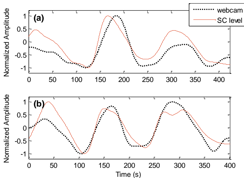
Fig.6. Results of the mental workload detection for the participant #11 (a) and #12 (b). Black plots correspond to the webcam-derived workload signal and red plots to the skin conductance level, derived from the raw electrodermal activity signal [24].
