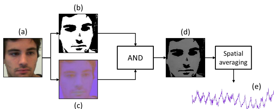
Fig.3. Algorithm overview. The face is automatically detected on each frame (a). Pixels that contain PPG information are isolated by a skin detection (b). The RGB color space is converted to the CIE L^*u^*v^* color space (c). The u^* frame is merged with the skin detection (d). A spatial averaging step is performed to transform a set of frames into a single raw signal (e).
