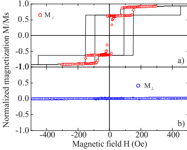
FIG. 2. (Color online) Normalized (a) longitudinal M_{\parallel} and (b) transverse M_{\perp} component of the magnetization (open symbols) as a function of field compared to the results of the micromagnetic calculation (lines).
