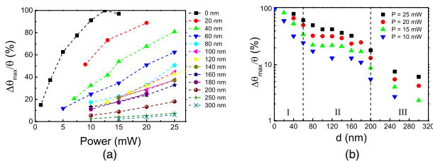
FIG. 3. (a) Power dependence of the induced Kerr rotation variation for different Cu thicknesses d . (b) Thickness dependence of the induced Kerr rotation variation for different power. Zone I corresponds to combined direct photon and hot electron excitation. In zone II, only hot electrons are responsible for the demagnetization. Zone III corresponds to a faster attenuation of the demagnetization.
