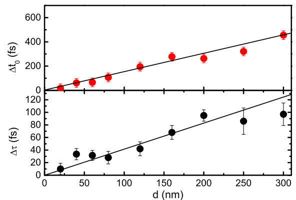
FIG. 2. (top) Cu thickness dependence of the induced time delay in the onset of demagnetization \Delta t_0 = t_0(d) - t_0(d=0) . The full line is a linear fit to the data. (bottom) Modification of the characteristic demagnetization time \Delta\tau(d) = \tau(d) - \tau(d=0) as a function of the Cu thickness d . The full line is a linear fit to the data.
