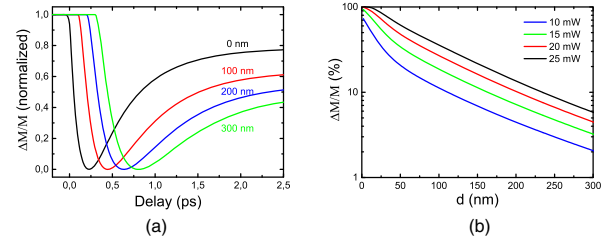
FIG. 4. (a) Simulation of ultrafast demagnetization for a laser power of 3.5 mW and different Cu thicknesses. (b) Simulation of the maximum demagnetization as a function of the Cu thickness for different laser power excitations. The hot electron attenuation length was set to 200 nm (see Supplemental Material [30] for details about the parameters used in the simulations).
