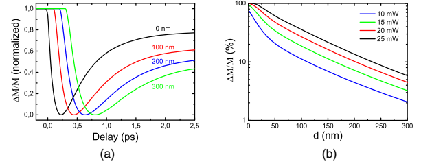
FIG. 4. (a) Simulation of ultrafast demagnetization for a laser power of 3.5 mW and different Cu thicknesses. (b) Simulation of the maximum demagnetization as a function of the Cu thickness for different laser power excitations. The hot electron attenuation length was set to 200 nm (see Supplemental Material [30] for details about the parameters used in the simulations).
