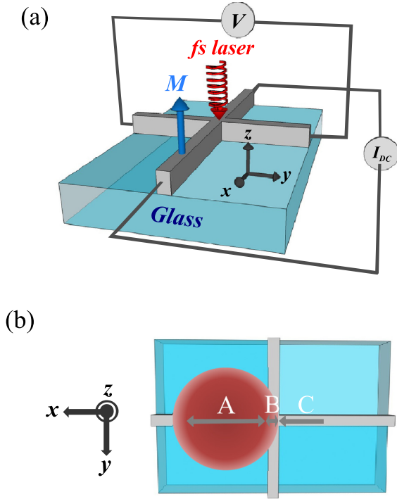
FIG. 1. (a) Schematic of the studied 5- \mu\text{m} -wide Hall crosses with perpendicular magnetization ( z axis); a dc current is injected along the x direction while the anomalous Hall voltage V_{\text{Hall}} is measured along the y direction with a temporal resolution of 1 \mu\text{s} . A fs laser beam with a FWHM of 60 \mu\text{m} illuminates the film plane along the z direction, at a fixed position about 40 \mu\text{m} from the center of the Hall cross along x direction. (b) Schematic representation of the different areas of the fs laser beam: “A” where multiple magnetic domains are obtained, “B” where AOS is obtained, and “C” where no change of magnetization is induced.
