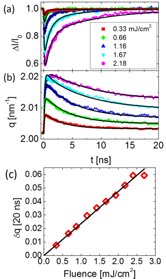
FIG. 3. (Color online) Time dependence of the loss in diffraction peak intensity (a) and change in q vector (b) as a function of pump fluence. Solid lines indicate fits to the model described in the text. (c) Remnant change in q as a function of pump fluence showing linear dependence consistent with sample heating.
