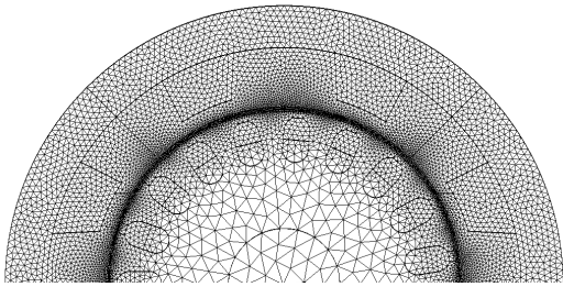
Figure 12. Description of the mesh in the entire machine.
