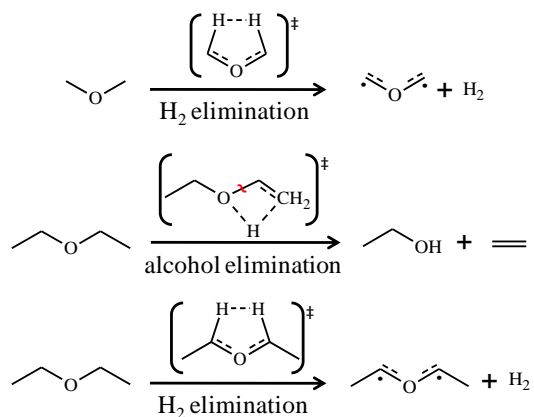
Figure 1: Pericyclic reactions of DME and DEE.
