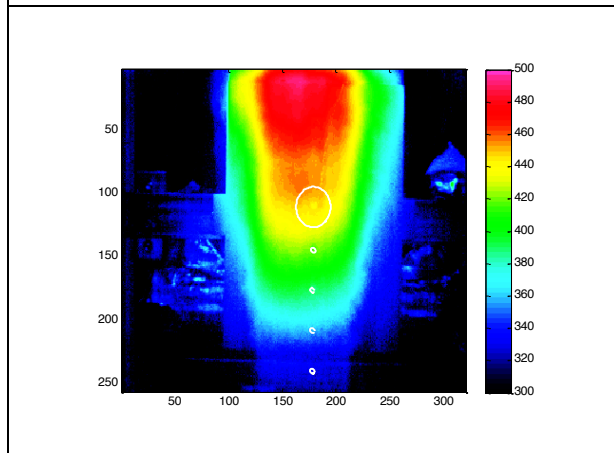
Figure 3: Typical IR image of the wall observed throughout the flame. Observation at 3.9 \mu\text{m} . Data converted in equivalent blackbody temperature (in K on the color bar).
