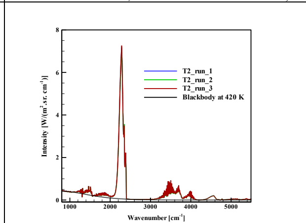
Figure 4: Typical IR spectrum. Intensities are plotted for three measurement tests. Case of turbulence 4%.
