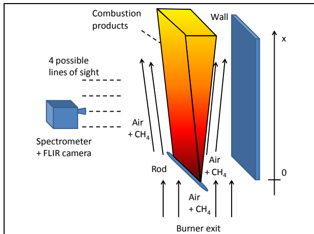
Figure 1: sketch of the setup
