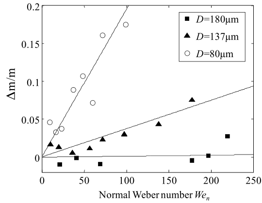
Fig. 9. Evolution of \Delta m/m as a function of the normal Weber number ( T_{wall} = 540^\circ\text{C} , f = 12\text{ kHz} ).
