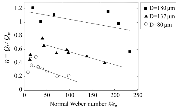
Fig. 10. Evolution of \eta as a function of the normal Weber number ( T_{wall} = 540^\circ\text{C} , f = 12\text{ kHz} ).
