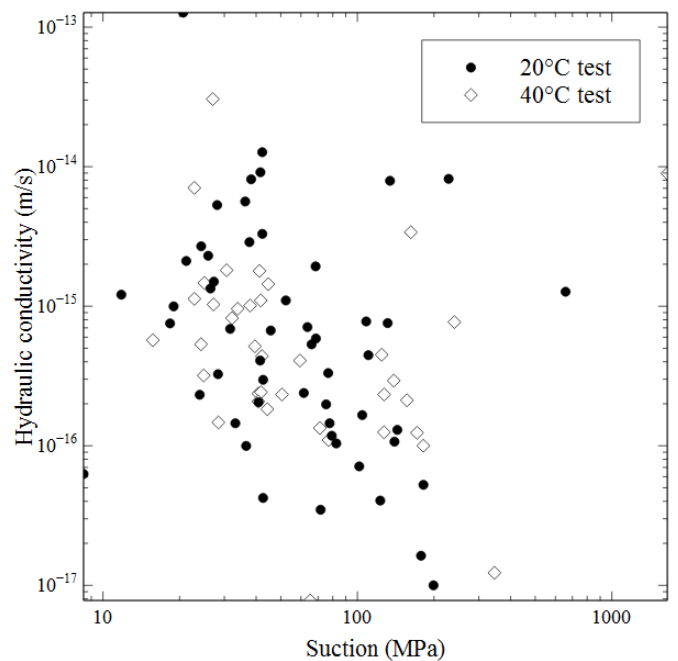
Figure 6. Unsaturated hydraulic conductivity curves derived from the tests.
