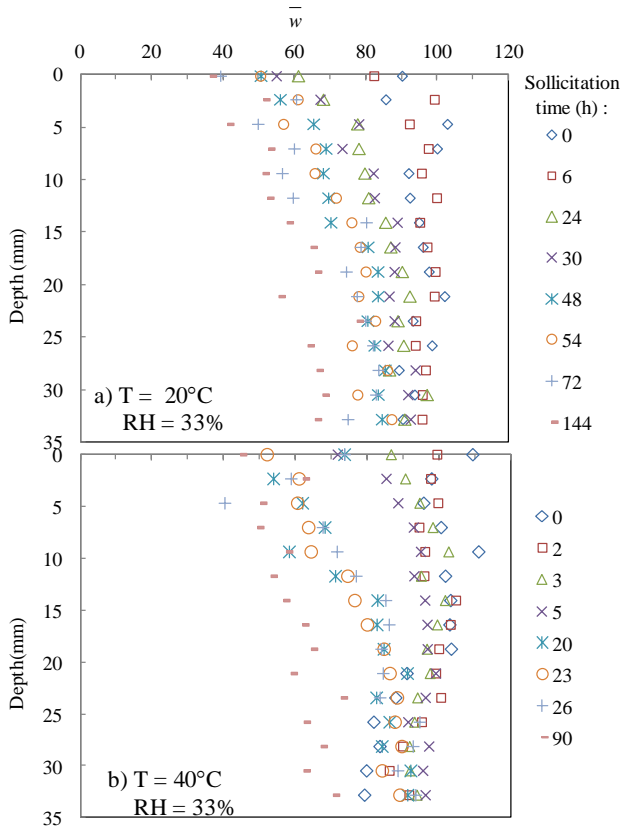
Figure 4. Drying tests on raw argillite submitted to a) T = 20^\circ\text{C} and \text{RH} = 33\% ; b) T = 40^\circ\text{C} and \text{RH} = 33\% .
