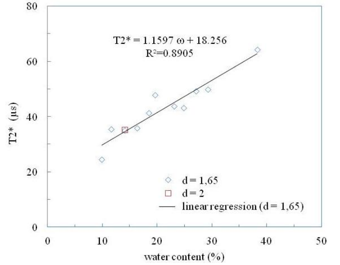
Figure 3. Calibration curve
