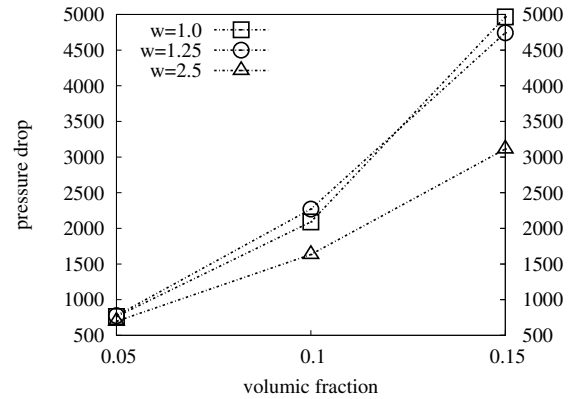
FIGURE 18. PRESSURE DROP THROUGH THE PARTICLES ARRAY FOR Re_p = 10.0 .
