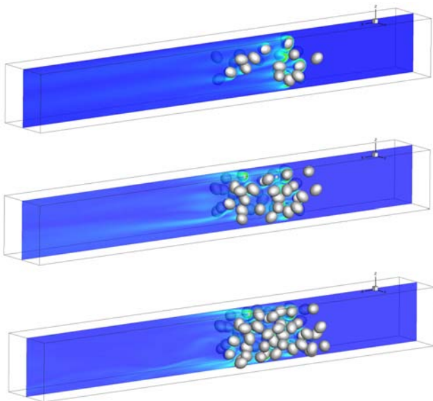
FIGURE 14. EFFECT OF THE SOLID VOLUME FRACTION ON THE NORMALIZED VORTICITY MAGNITUDE. NON-SPHERICAL PARTICLES ARRAY FOR w = 1.25 AND Re_p = 100.0 . FROM TOP TO BOTTOM: \alpha_p=5\% , 10% AND 15%.
