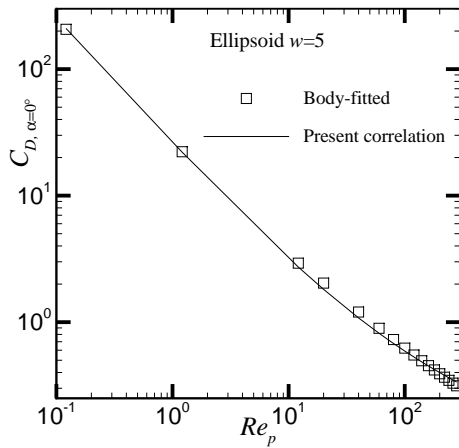
FIGURE 8. COMPARISON BETWEEN COMPUTATIONAL DRAG COEFFICIENT WITH THE PRESENT CORRELATION AT \alpha = 0^\circ .
