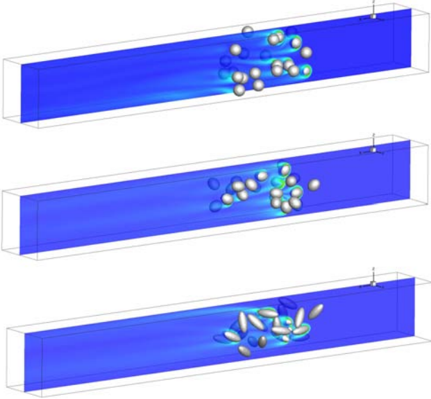
FIGURE 16. EFFECT OF THE ASPECT RATIO ON THE NORMALIZED VORTICITY MAGNITUDE FOR THE NON-SPHERICAL PARTICLE FOR \alpha_p = 5\% AND Re_p = 100 . FROM TOP TO BOTTOM: w=1.0 , 1.25 AND 2.50 .
