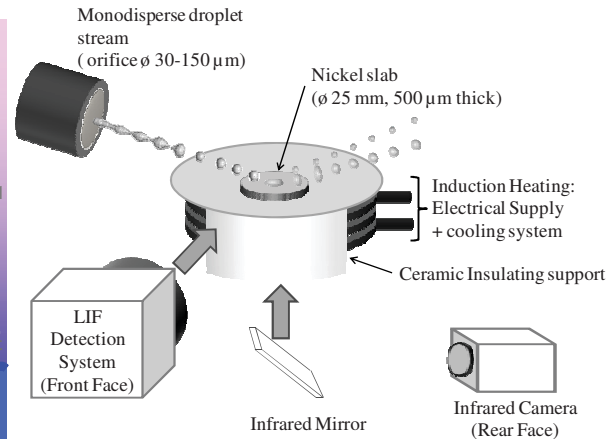
Figure. 13: Temperature measurement
