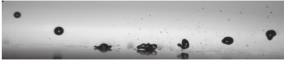
Figure 14: droplet-wall interaction in the bouncing regime (Weber < 40)
