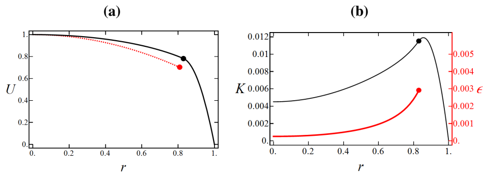
Figure 1 : Mean fields for R = 3000 , as a function of the dimensionless radius r . The disks show the location of the radius r_0 , given by (13), where the boundary conditions apply. (a) : Mean velocity U(r) after the spectral computations (full line) and initial guess (dashed line). (b) : Turbulence kinetic energy K(r) (thin line) and dissipation rate \epsilon(r) (thick line) after the spectral computations.
