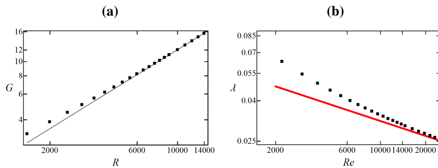
Figure 4 : (a): Pressure gradient vs R (squares) and power law (24) (continuous line). (b): Friction factor vs Re (squares) and Blasius correlation (22) (continuous line).
