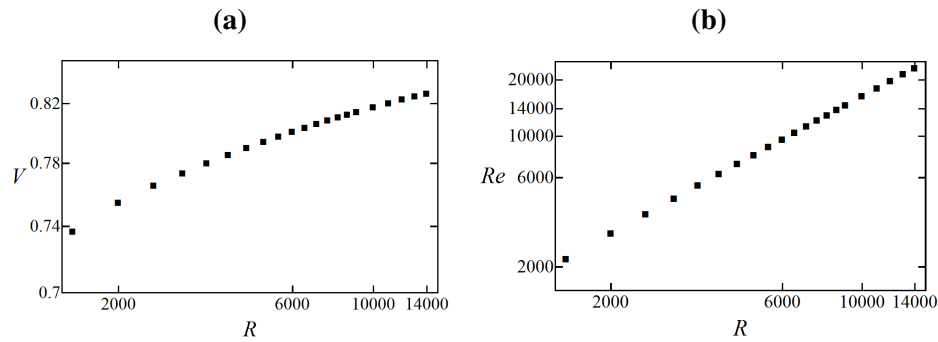
Figure 3 : Global values vs the centerline velocity Reynolds number R . (a): Bulk velocity (log-log scale). (b): Bulk velocity Reynolds number Re .
