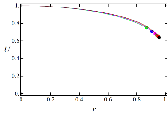
Figure 2 : Mean velocity U(r) for R = 4000 to 14000 by steps of 2000 . The disks indicate the radius r_0 given by (13), that increases when R increases.
