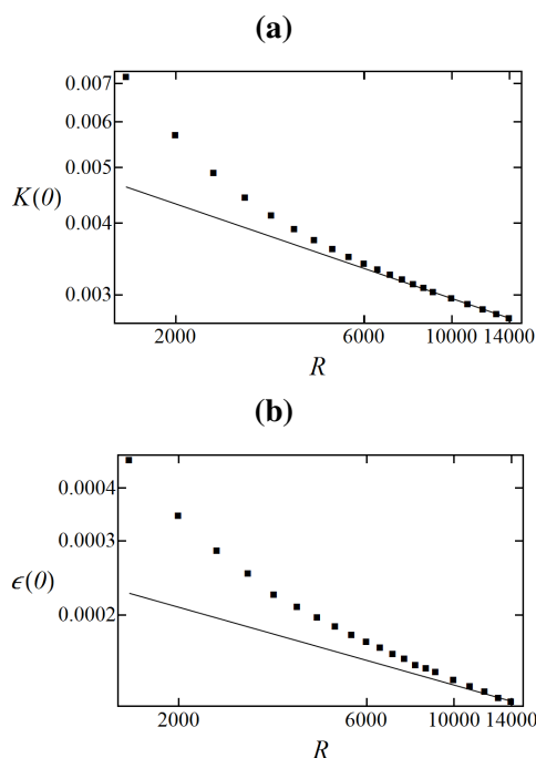
Figure 5 : Values of the turbulent fields at the center of the pipe, r = 0 , vs R : the squares show the numerical results and the full lines the power laws (26). (a): Kinetic energy. (b): Dissipation rate.
