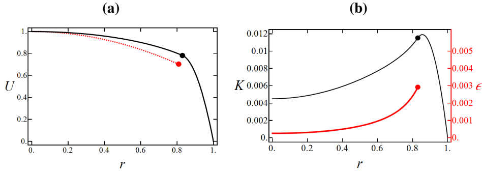
Figure 1 : Mean fields for R = 3000 , as a function of the dimensionless radius r . The disks show the location of the radius r_0 , given by (13), where the boundary conditions apply. (a): Mean velocity U(r) after the spectral computations (full line) and initial guess (dashed line). (b): Turbulence kinetic energy K(r) (thin line) and dissipation rate \epsilon(r) (thick line) after the spectral computations.
