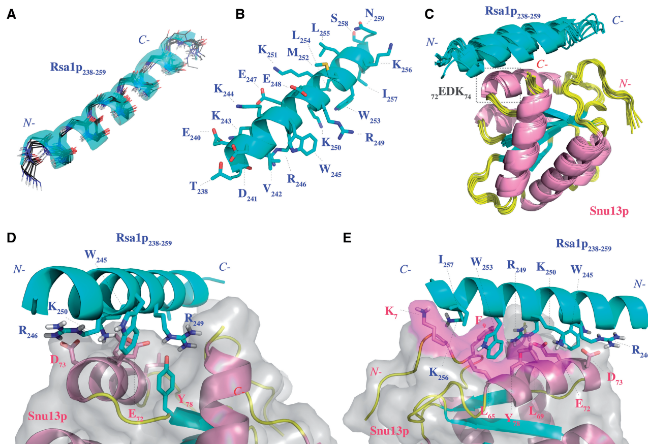
Figure 8. The Rsa1p 238–259 NMR structure and modeling of the Snu13p–Rsa1p interaction show both electrostatic and hydrophobic components at the protein–protein interface. (A) Backbone superimposition of the 10 best structures of Rsa1p 238–259 . (B) Side-chains representation of the lowest energy Rsa1p 238–259 structure. The helical conformation is highlighted using a cartoon representation. The hydrogen atoms are not represented. (C) Ribbon representation of the 10 3D models with the lowest haddock score resulting from the docking of the lowest energy NMR structure of Rsa1p 238–259 on the X-ray structure of Snu13p. (D) Ionic interaction network between R 246 , R 249 and K 250 in Rsa1p 238–259 and E 72 and D 73 in Snu13p. (E) Highlight of the Snu13p pocket hosting the W 253 in Rsa1p 238–259 . The figures have been done with PyMOL software (66).
