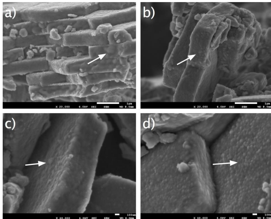
6 7 Fig. 2. SEM micrographs of the pre-extraction (a, c) and post-extraction (b, d) nacre powder, SEI 8 mode, 4kV. The organic matrix at lateral surface (arrow in a and b) and frontal surface (arrow in c 9 and d) of nacre tablet is extracted by ethanol (b and d), without modification to nacre micro- 10 architected structures. Scale bar corresponds to 1 μm (a, b) and 100 nm (c, d) respectively.
