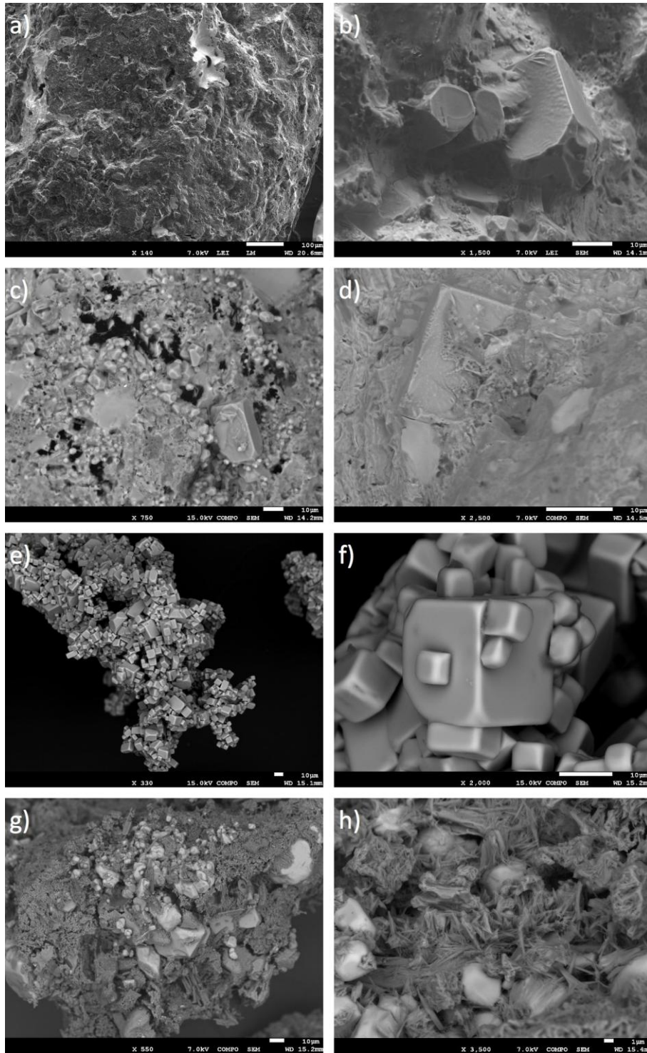
2 Fig. 8. SEM micrographs of (ab) ESM, (cd) ESMc, (ef) ESMa and (gh) F6. (a) ESM is a mixture of 3 organic matrix and mineral crystals, (b) and the crystals are embedded into the organic matrix, but 4 easily recognized; (c) ESMc is also a mixture like ESM, but the crystals are separated with the matrix, 5 (d) when focused onto the matrix, the crystals are difficult to recognize; (e,f) ESMa is nearly composed 6 of pure and regular crystals, no matrix is observed; (g,h) F6 is majorly made of organic matrix, loose
