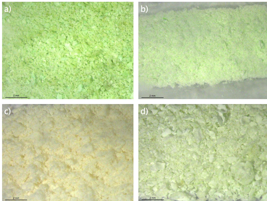
2 Fig. 3. Optical micrographs: (a) ESM, (b) ESMc, (c) ESMa and (d) ESME. ESM, ESMc and ESME share a 3 green appearance, while ESMa appears canary. ESMc and ESMa present a finer appearance than ESM. 4 LEICA microscope (M80, obj x1). Scale bar corresponds to 2 mm.
