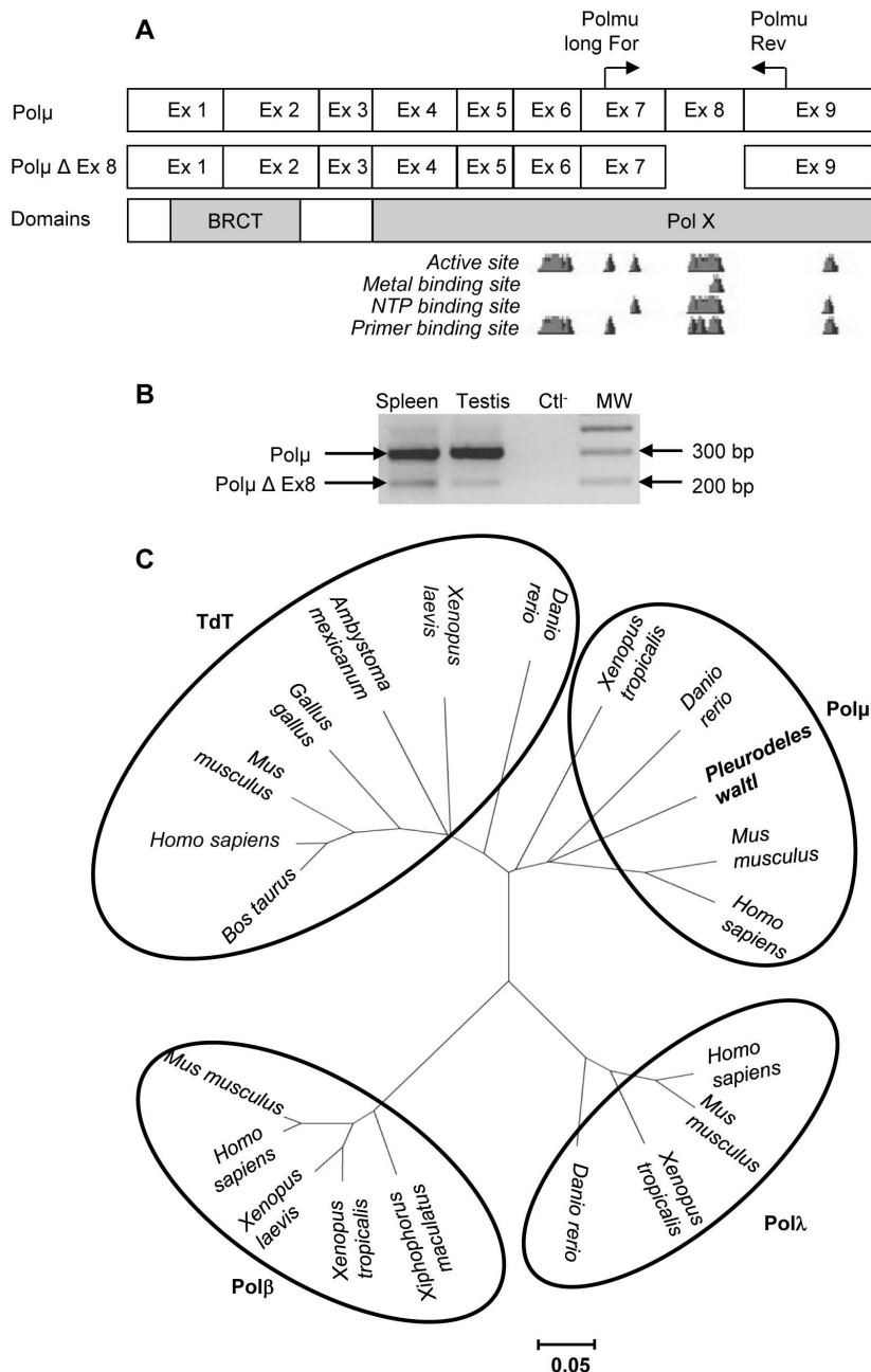
Figure 1. Pleurodeles waltl DNA polymerase \mu . Schematic representation of P. waltl Polμ mRNAs ( A ). The short variant (Polμ Δ Ex 8) presents a 103 bp deletion corresponding to exon 8. This deletion removes one part of the active site of the protein. The BRCT (breast cancer suppressor protein carboxy-terminal) and the Pol X domain, which contains the active site, are required for Polμ function. Polμ variants were amplified using primers indicated by horizontal arrows ( B ). Quantification of the obtained PCR products using a Gel Doc 2000 and the Quantity One v.4.3.1 software (Bio-Rad, Hercules, CA, USA) indicates that the short isoform represents 16% and 6% of the Polμ transcripts in the spleen and testis of P. waltl , respectively. Ctl - = negative control. MW = 100 bp DNA ladder. A cladogram was then constructed by neighbor joining ( C ) supported with 1000 bootstrap replications using the MEGA4 software ( http://www.megasoftware.net/ ) and the following sequences: Terminal deoxynucleotidyl transferase (TdT); Bos taurus (DAA14763), Homo sapiens (BAB72001), Mus musculus (NP_001036693), Gallus gallus (NP_990720), Ambystoma mexicanum (AA092254), Xenopus laevis (NP_001079251), Danio rerio (AAS89780). Polymerase beta; Mus musculus (NP_035260), Homo sapiens (NP_002681), Xenopus laevis (NP_001081643), Xenopus tropicalis (AAH74537), Xiphophorus maculatus (AAU11319). Polymerase lambda; Danio rerio (NP_998408), Xenopus tropicalis (NP_001093716), Mus musculus (NP_064416), Homo sapiens (NP_001167555). Polymerase mu; Homo sapiens (NP_037416), Mus musculus (NP_059097), Danio rerio (NP_956542), Xenopus tropicalis (NP_001164987), Pleurodeles waltl (HE583591). The scale bar corresponds to the evolutionary distance. doi:10.1371/journal.pone.0069647.g001
