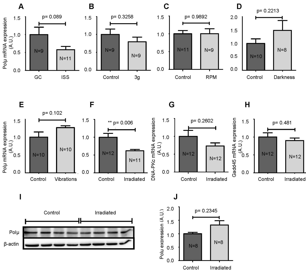
Figure 3. Effects of spaceflight conditions. Polμ mRNAs were quantified in larvae that developed in microgravity in the ISS (A), in hypergravity (B), in the RPM to simulate microgravity (C) or in the dark (D). The same study was performed with larvae subjected to a mechanical stress (E) or the ISS radiation environment (F). The effects of space radiation on DNA-PKc (G) and Gadd45 (H) mRNAs and on the amount of Polμ protein (I and J) were also investigated. Western blot results were analyzed and quantified by densitometry using a Fusion Fx7 imaging system (Vilber Lourmat, Marne-la-Vallée, France) and Polμ expression was normalized to β-actin (J). Each lane of the western blot contains proteins from 3 larvae. Results are expressed as the mean ± SEM. "A.U." stands for "arbitrary units". doi:10.1371/journal.pone.0069647.g003
