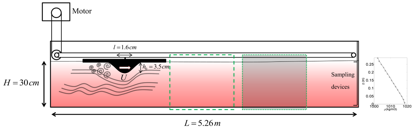
Figure 1. Experimental setup (not to scale). The tank is filled with a linear salinity gradient (inset at right). Red dye is a passive tracer of salt. (middle) The rectangle in green broken line indicates the area of density field measurements and (right) the shaded green rectangle indicates the location of shadowgraph photographs.
