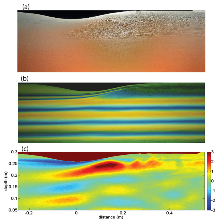
Figure 5. (a) Shadowgraph; (b) dyed isopycnal layers and (c) density perturbations for flow over the wider ridge at Fr_h = 0.44 , Re = 1700 (exp28).
