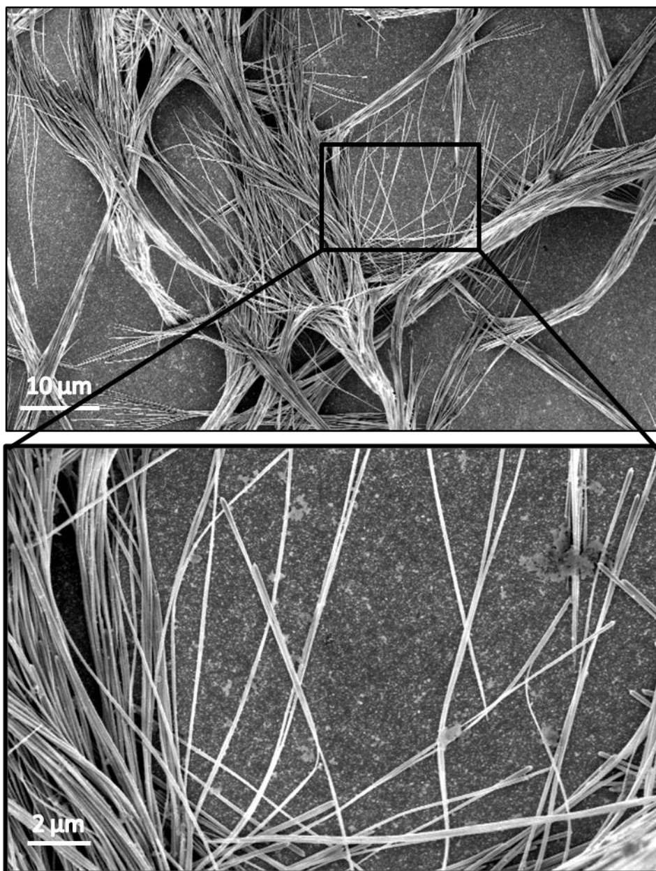
Figure 6 : SEM images of Te nanowires deposited at C_{1^{st}} peak potential in pure EOPipTFSI. [Te^{IV}] = 5 \text{ mM} . T = 100^{\circ}\text{C} , Q = 2 \text{ C/cm}^2 , Pt-coated glass slide.
