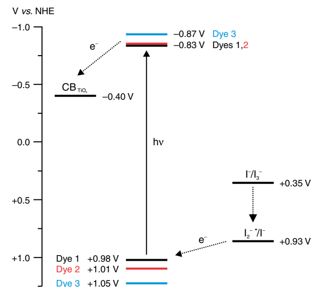
Figure 10. Energy diagram for the dyes (1) cis -[Ru(Me 4 -phen)(dcbH 2 )(NCS) 2 ]; (2) cis -[Ru(Me 2 -phen)(dcbH 2 )(NCS) 2 ] and (3) cis -[Ru(phen)(dcbH 2 )(NCS) 2 ].
