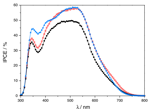
Figure 8. Photocurrent action spectra of cis -[Ru(Me 4 -phen)(dcbH 2 )(NCS) 2 ] (●), cis -[Ru(Me 2 -phen)(dcbH 2 )(NCS) 2 ] (□) and cis -[Ru(dcbH 2 )(NCS) 2 ] 2- (▲).
