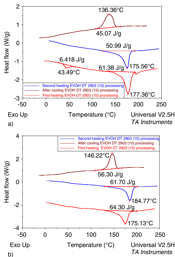
Figure 8 Comparison between the DSC curves obtained for an EVOH film of 10 \mu\text{m} a) before conditioning and b) after conditioning. First heating (red), second heating (blue), after cooling (black).
