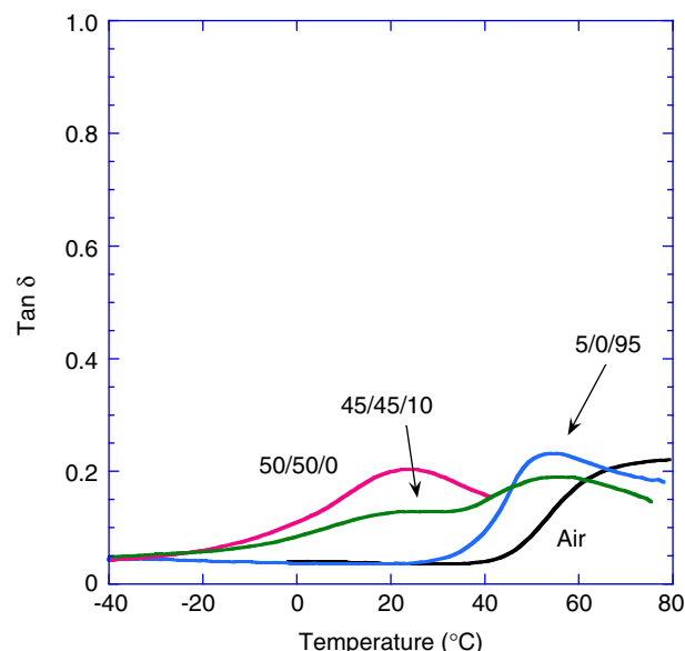
Figure 13 Variation of the loss factor \tan \delta of an EVOH film of 60 \mu\text{m} after its conditioning in model fuel mixtures ethanol/ i -octane/toluene with increasing ethanol contents.
