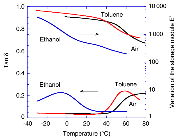
Figure 12 Variation of the loss factor \tan \delta and of the storage modulus E' of an EVOH film of 60 \mu\text{m} after its conditioning in pure toluene and pure ethanol.
