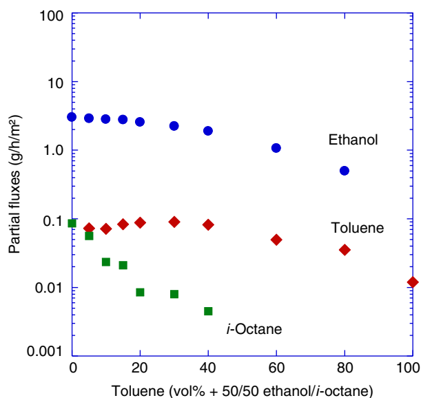
Figure 7 Partial fluxes of a preconditioned EVOH film of 24 \mu\text{m} for model fuel mixtures ethanol/ i -octane/toluene ( x/x/y vol%) corresponding to the toluene tie line at 50°C.
