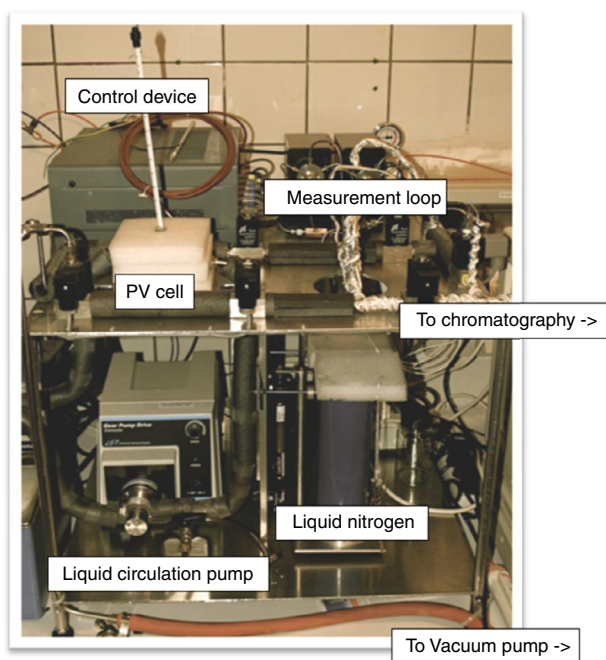
Figure 2 Photograph of the automated permeameter.
