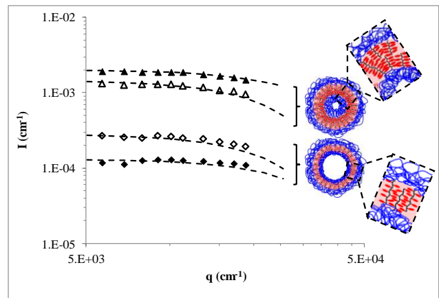
Figure 3. Scattered intensity (I) of vesicles as function of scattering vector (q) of: (▲) C_3^{\text{DMSO}} , (Δ) C_3^{\text{THF}} , (◆) C_4^{\text{DMSO}} and (◇) C_4^{\text{THF}} . Dashed lines are fits to equation S4. Schematic representations of vesicles and of their membranes are given.
