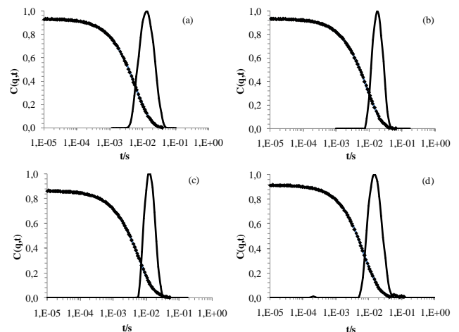
Figure 1. Autocorrelation functions C(q,t) as a function of time and corresponding relative distribution of relaxation times recorded at a scattering wave vector q=4.6 \times 10^{-3} \text{ nm}^{-1} ( \theta=20^\circ ) for different nanostructures dispersed in water. (a) C 3 DMSO , (b) C 3 THF , (c) C 4 DMSO , (d) C 4 THF .
