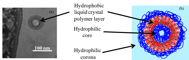
Figure 2. (a) Cryo-TEM image of polymersome obtained in water after dialysis of Dex-g 5 -PADEGChol 79 dispersed in THF(case of C_3^{\text{THF}} ). (b) schematic representation of such vesicle.
