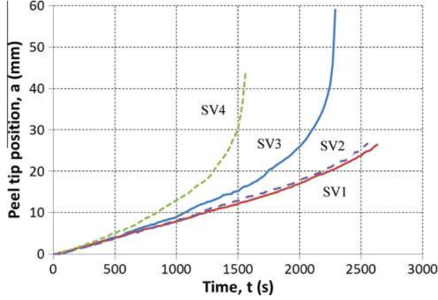
Fig. 8. Peel tip position, a , as a function of time, t , for varying stage stop times for separate experiments with tape of variable width.
