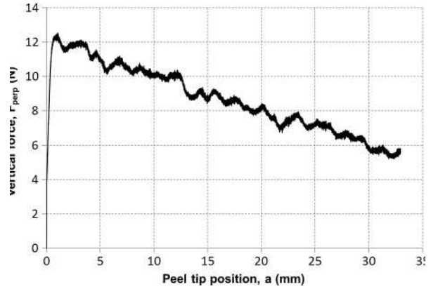
Fig. 9. Vertical component of the peel force ( F_{perp} ) vs. peel tip position, a , for a displacement controlled peel experiment on a variable width tape (Eq. (17)).
