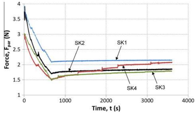
Fig. 7. Measured force parallel to the substrate, F_{par} as a function of time, t , for experiments of variable string stiffness and various combinations of F_{perp} and F_{par0} . The corresponding tip position, a , as a function of time is shown in Fig. 6.
