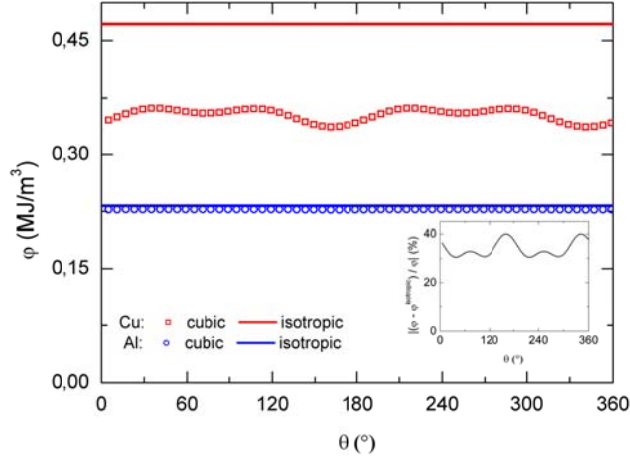
Figure 9. Evolution of the stored elastic energy density \phi in crystal II with the angle \theta for \gamma = 0.01 . Crystal I remains fixed while crystal II can rotate around (O, x_2) by the angle \theta . Inset: relative error made by the isotropic approximation for Cu.
