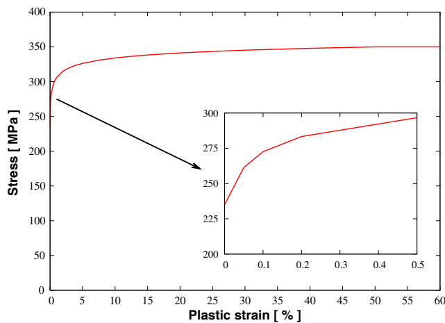
Fig. 4 Hardening law described as a piecewise linear function
