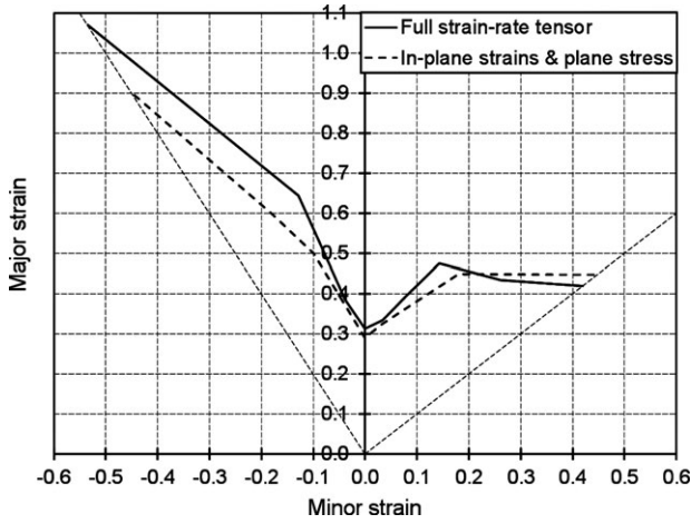
Figure 5. Simulated FLDs associated with linear loading paths for the IF-Ti single-phase steel obtained with the bifurcation-EPSC model: two different ways to prescribe the strain paths.
