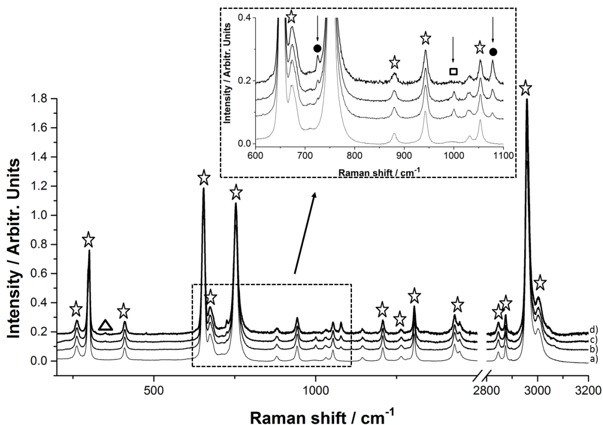
Figure 3. Raman spectra recorded at open-circuit potential at the macroscopic liquid/liquid interface constituted between 5 mM NaCl aqueous solution and: a) DCE, b) 10 mM BTPPA + TPBCl - in DCE, c) 10 mM BTPPA + TPBCl - and 14 mM CTA + TPBCl - in DCE and d) 53 mM CTA + TPBCl - in DCE. Raman bands marked with (□) were assigned to BTPPA + , with (●) to TPBCl - , with (★) to DCE and with (▲) to CTA + .
