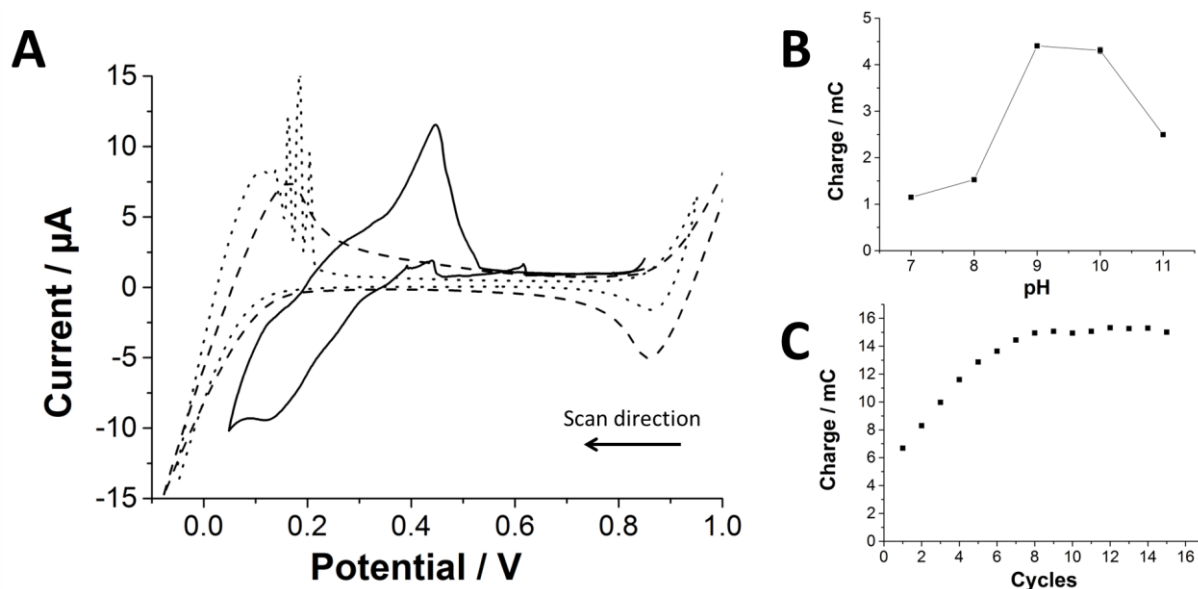
Figure 1. (A) Cyclic voltammograms (CV) in the presence of 50 mM TEOS, and in the presence of 1.5 mM \text{CTA}^+ (solid line); CVs in the absence of either \text{CTA}^+ (dashed line) or TEOS (dotted line) in the electrochemical cell; \nu = 5 \text{ mV s}^{-1} . (B) Influence of pH on the reverse peak charge. The charge is the average of the last five values of 15 consecutive CVs. ( [\text{CTA}^+]_{\text{org.}} = 3 \text{ mM} , [\text{TEOS}]_{\text{aq.}} = 300 \text{ mM} ). (C) Reverse peak charge as a function of the number of cycles ( [\text{CTA}^+]_{\text{org.}} = 14 \text{ mM} and [\text{TEOS}]_{\text{aq.}} = 50 \text{ mM} ; \nu = 5 \text{ mV s}^{-1} ).
