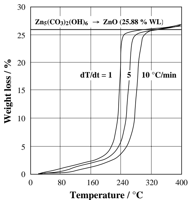
Fig. 5 : Treatment of RFS at different heating rates.
