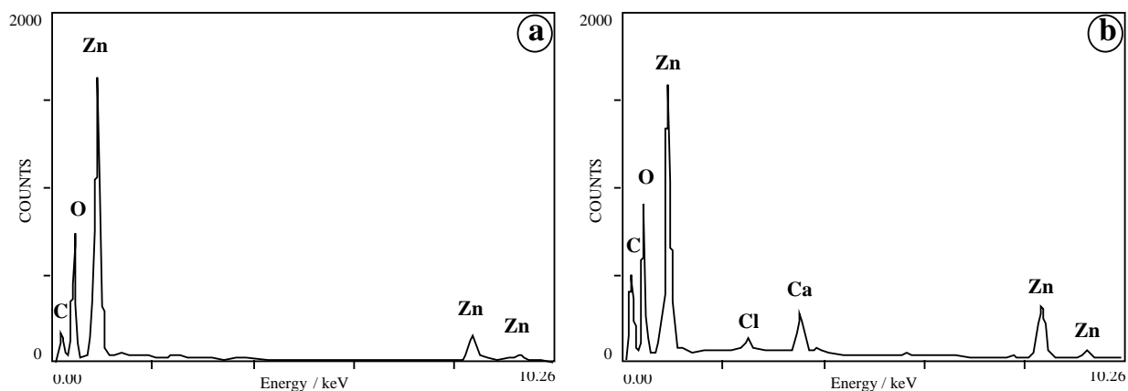
Fig. 2 : SEM-EDS spectra of the zinc carbonate hydroxide samples
