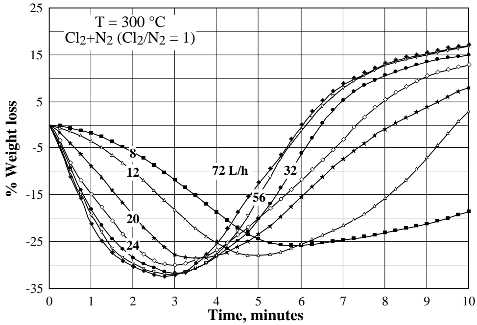
Fig. 7 : Isotherms of chlorination of HGC with \text{Cl}_2+\text{N}_2 using various gas flow rates.
