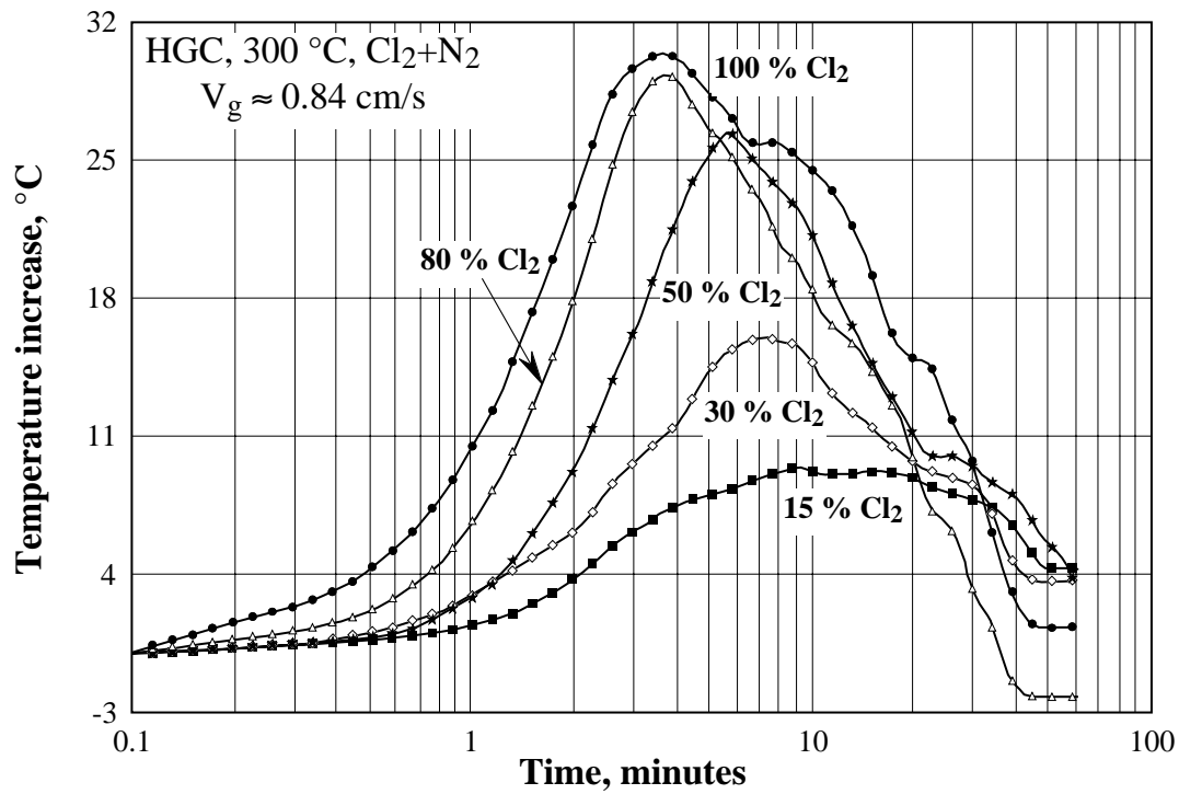
Fig. 21 : Increase of temperature during the chlorination of HGC in a horizontal experimental set using different chlorine contents in \text{Cl}_2 + \text{N}_2 gas mixture.
