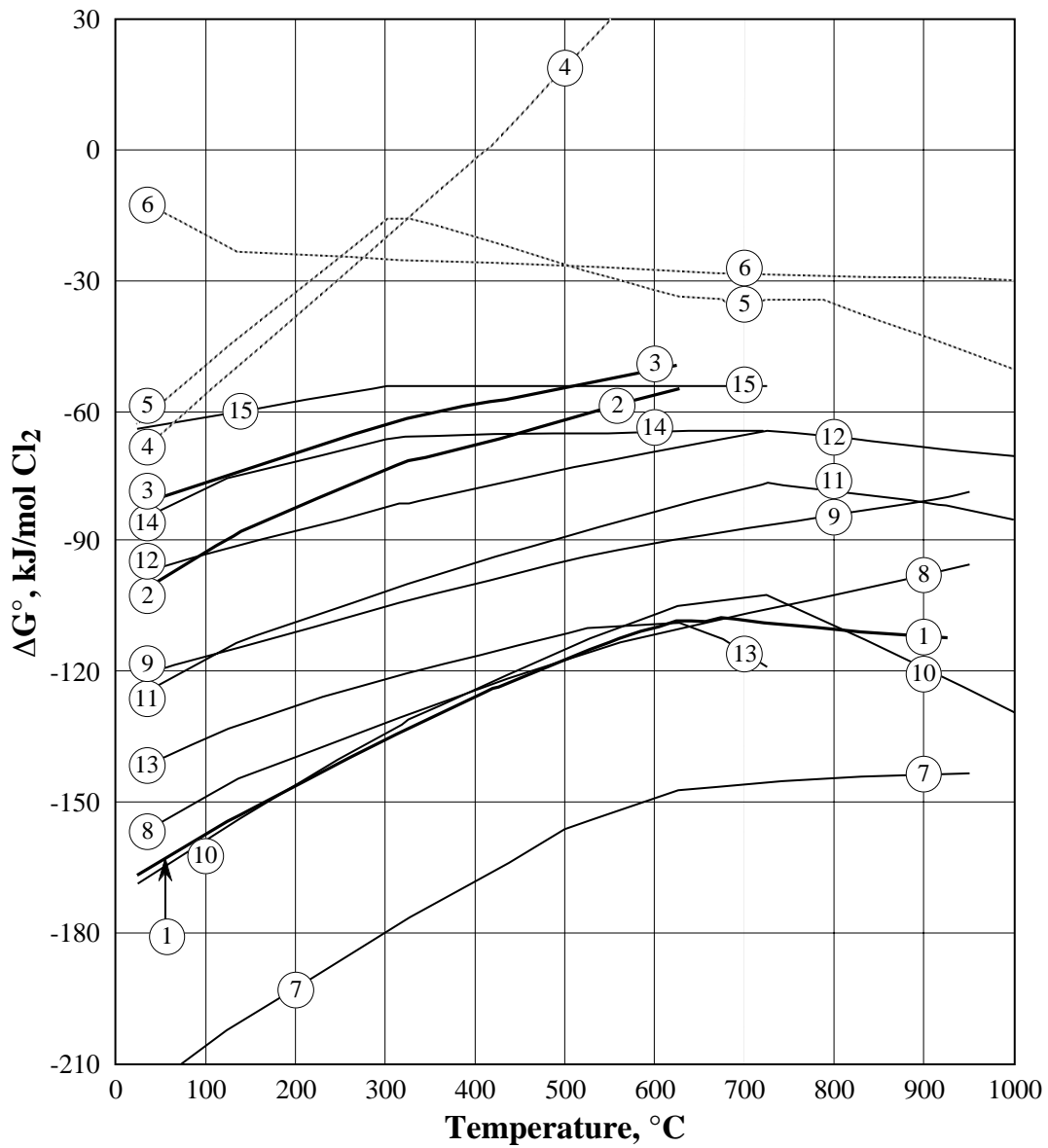
Fig. 3 : Evolution of the standard free energy changes ( \Delta G^\circ ) as a function of temperature for the chlorination of the compounds contained in the chalcopryrite concentrates [14,15] .
