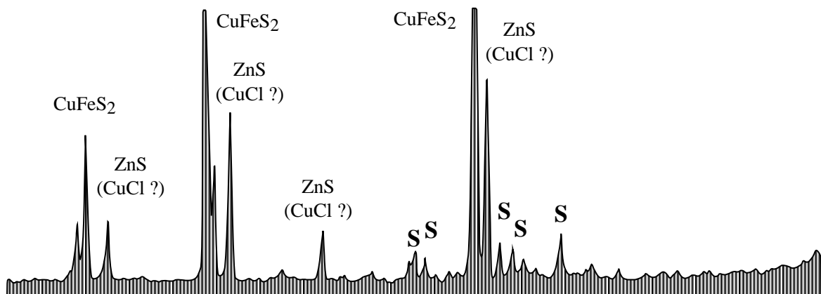
Fig. 20 : XRD result of the residue obtained during the HGC chlorination at 200 °C for 10 minutes (leached at \text{pH} \approx 2 ).
