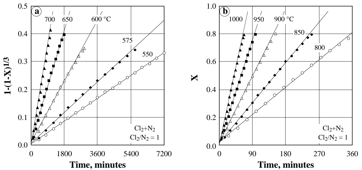
Fig. 6- Mathematical fitting of the chlorination data at (a) T \leq 700^\circ\text{C} using Eq. 14 and (b) T \geq 800^\circ\text{C} using Eq. 12.
