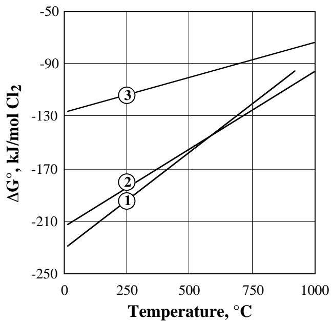
Fig. 2 - Standard free energy change of Cr 2 O 3 carbochlorination reactions.
