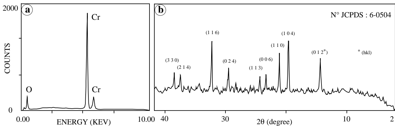
Fig. 1- Results of (a) SEM and (b) XRD analysis of Cr 2 O 3 sample.
