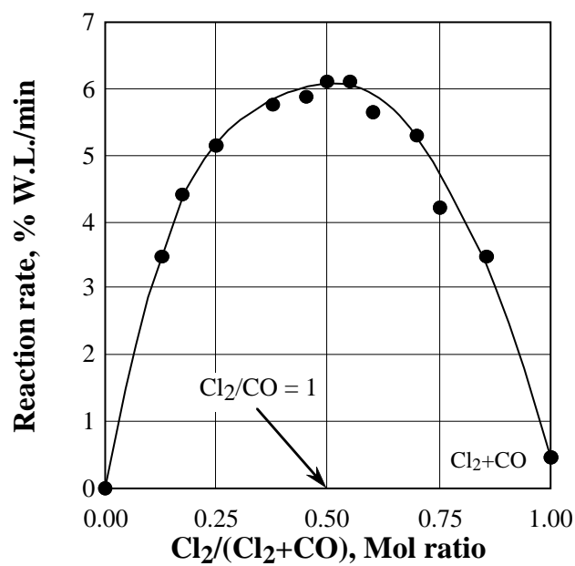
Fig. 12- Effect of \text{Cl}_2/(\text{Cl}_2+\text{CO}) ratio on the \text{Cr}_2\text{O}_3 carbochlorination rate at 800\text{ }^\circ\text{C} .
