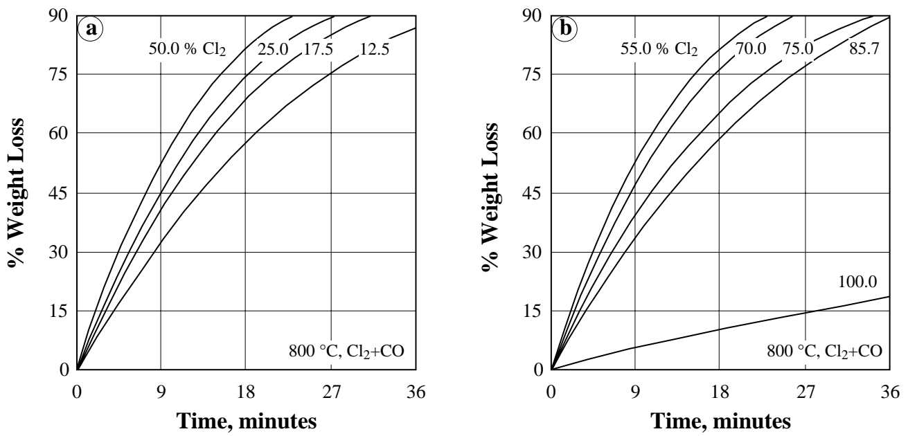
Fig. 11- Isotherms of carbochlorination of \text{Cr}_2\text{O}_3 at 800\text{ }^\circ\text{C} with \text{Cl}_2+\text{CO} for (a) 12.5 \leq \text{Cl}_2 \leq 50.0 pct and (b) 55.0 \leq \text{Cl}_2 \leq 100.0 pct.
