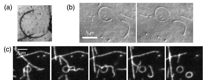
FIG. 1. (a)–(c) Mysterious ring formation of microtubules gliding on a kinesin motor carpet (from [18], [22], and [24]).
