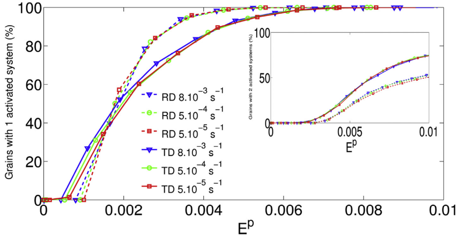
Fig. 11. Proportion of grains with one activated system (i.e., grains with \gamma > 0.004 on the most active system). Inset: proportion of grains with two activated systems (i.e., grains with \gamma > 0.004 on the second most active system).
