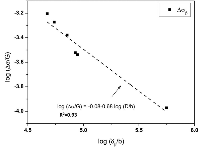
Fig. 10. Relationship between incremental stress normalized by the shear modulus and \beta -subgrain size normalized by the burgers vector of samples deformed above T_\beta .
