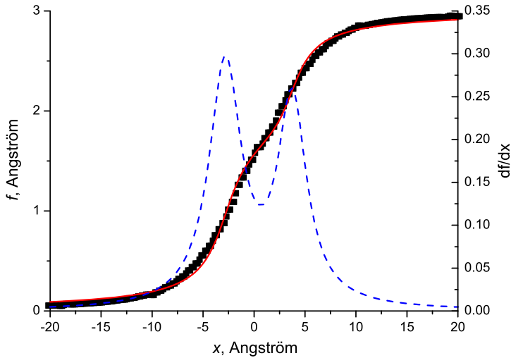
Figure 9. (colour online) Core structure of 60^\circ dislocation. Disregistry function f(x) and associated Burgers vector density \rho = df(x)/dx (dotted line) are plotted in (0001) plane.
