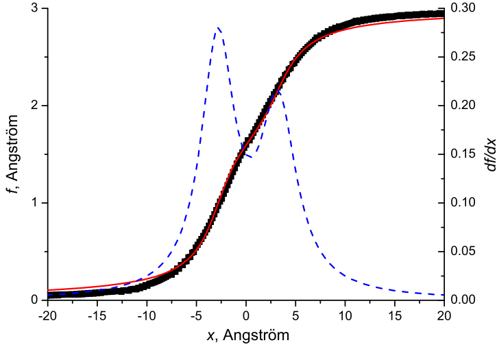
Figure 8. (colour online) Core structure of 30^\circ dislocation. Disregistry function f(x) and associated Burgers vector density \rho = df(x)/dx (dotted line) are plotted in (0001) plane.
