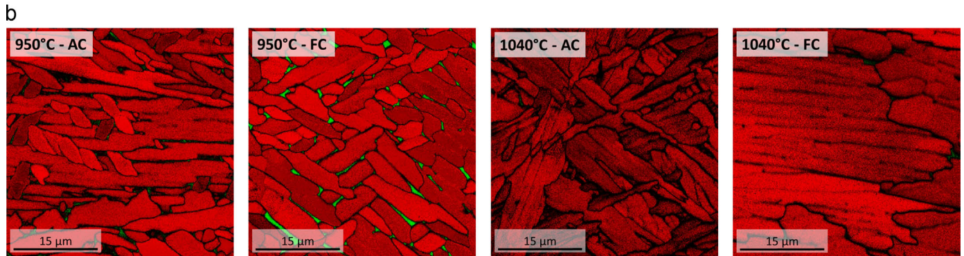
Fig. 8. (a) X-ray diffraction of as-built and heat-treated electron beam melted cubes; (b) \alpha/\beta phase distribution images of heat-treated electron beam melted cubes, measured using EBSD mapping. The \alpha phase and the \beta phase are highlighted in red and green, respectively. (For interpretation of the references to color in this figure legend, the reader is referred to the web version of this article.)
