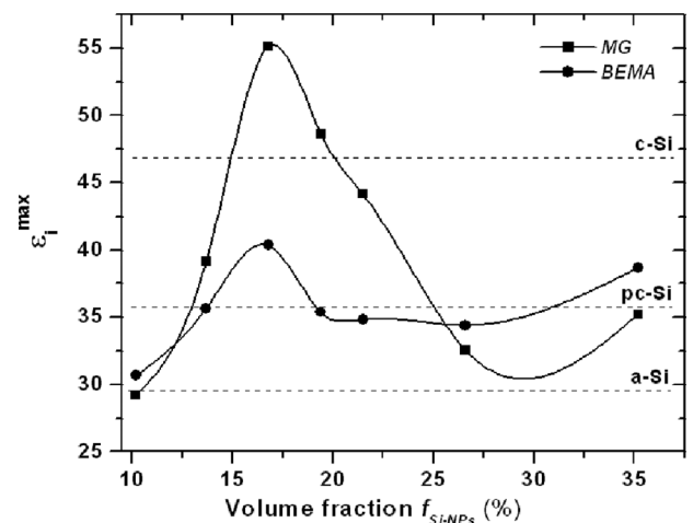
FIG. 4. Evolution of the amplitude \epsilon_i^{\max} of the \epsilon_i peak derived from MG and BEMA for the samples studied in this work. The values of \epsilon_i^{\max} related to the main peak of a-Si , pc-Si , and c-Si are also provided as references (dashed lines). The spline lines connecting each data are guides for the eye.
