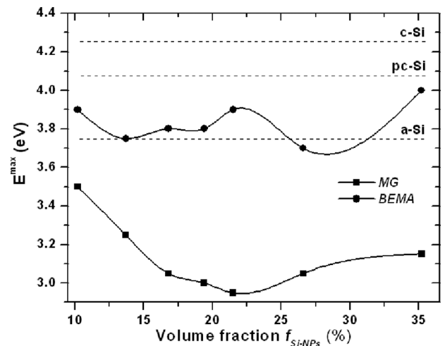
FIG. 5. Evolution of the position E^{max} of the \epsilon_i peak obtained from MG and BEMA for the samples investigated in this work. The values of E^{max} related to the main peak of amorphous Si ( a-Si ), polycrystalline Si ( pc-Si ) and crystalline Si ( c-Si ) are also provided as references (dashed lines). The spline lines connecting each data are guides for the eye.
