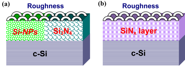
FIG. 3. The two optical models employed for the derivation of the dielectric function of the Si-NPs and evaluation of their size dispersion. The optical model (a) describes the same layer as a composite \{Si-NPs + Si_3N_4\} film by taking into account the optical contributions of the Si-NPs and the silicon nitride matrix distinctly. The optical model (b) considers the silicon-rich silicon nitride SiN_x film as a homogeneous layer. The same optical models as those we used in Ref. 34 are employed.
