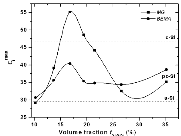
FIG. 4. Evolution of the amplitude \epsilon_i^{max} of the \epsilon_i peak derived from MG and BEMA for the samples studied in this work. The values of \epsilon_i^{max} related to the main peak of a-Si , pc-Si , and c-Si are also provided as references (dashed lines). The spline lines connecting each data are guides for the eye.
