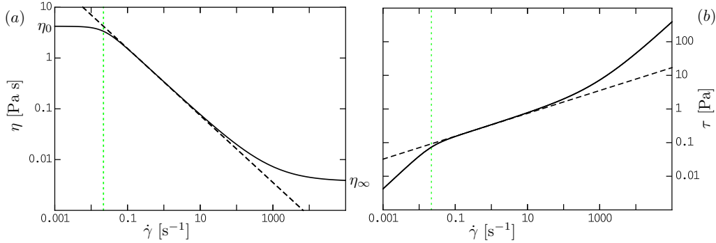
FIGURE 1. (Colour online) Flow curves of the 0.125% PAA fluid studied by Escudier et al. (2009): (a) viscosity (b) shear stress vs shear rate. Continuous curves, Carreau's model (2.6) with \eta_0 = 4.22 Pa s, \eta_\infty = 0.00372 Pa s, \lambda_C = 45.8 s, n_C = 0.34 ; dashed lines, power-law model; vertical dotted lines, characteristic shear rate \dot{\gamma} = 1/\lambda_C for the onset of shear-thinning.
