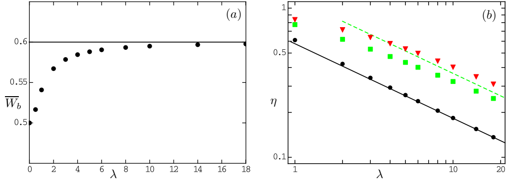
FIGURE 3. (Colour online) For n_C = 0.5 . (a): \circ , bulk velocity of the base flows; full line, power-law fluid bulk velocity of the base flows. (b): \circ , wall viscosity of the base flows; full line, power-law fluid wall viscosity of the base flows; \square , bulk average mean viscosity of the base flows; dashed line, power-law fluid mean viscosity of the base flows; \nabla , bulk average mean viscosity of the critical waves discussed in §5.3.
