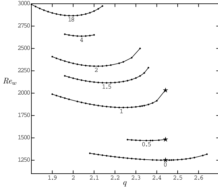
FIGURE 8. For n_C = 0.5 . Onset curves Re_w(q, 0.5, \lambda) for various values of \lambda , as indicated under the critical point of each curve; \star , solutions found by RPN2010.
