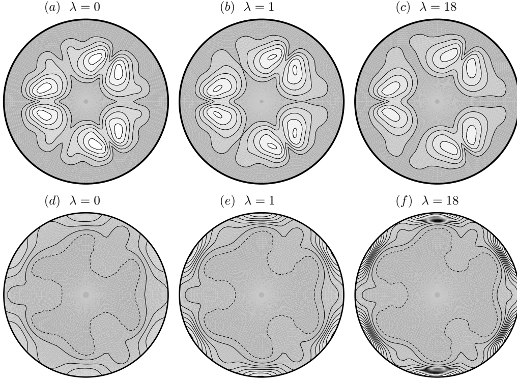
FIGURE 12. For n_C = 0.5 , for various values of \lambda as indicated. (a, b, c): rms axial velocity w'(r, \theta) ; continuous lines, 5 regularly spaced contours w' = 0.025\bar{W} to 0.125\bar{W} ; dark gray (resp. light gray), low (resp. high) values. (d, e, f): \langle \Gamma_2 \rangle_z ; dashed line, first iso contour \Gamma_2 = 0.5 ; continuous lines, 10 regularly spaced contours \Gamma_2 = 1.5 (near the center) to 15 (near the pipe wall).
