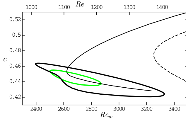
FIGURE 6. (Colour online) For n_C = 0.5 , \lambda = 2 . Black curves: three branches of wave solutions for q = 2.28 : thick line, lower branch; thin continuous line, intermediate branch; thin dashed line, higher branch. Gray (green online) curve: lower branch of wave solutions for q = 2.32 .
