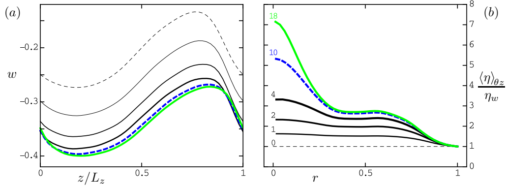
FIGURE 13. (Colour online) For n_C = 0.5 , for the critical waves corresponding to the values of \lambda indicated in figure (b). (a): axial velocity w = v_z - W_b at r = 0.59 , \theta = 1.29 . (b): ratio of the viscosity averaged over \theta and z to the wall viscosity.
