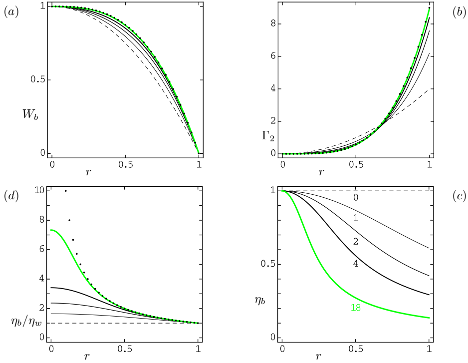
FIGURE 2. (Colour online) Properties of the laminar base flows for n_C = 0.5 and different values of \lambda as indicated below each curve of figure (c). (a): Axial velocity. (b): Rate-of-strain intensity. (c): Viscosity. (d): Ratio of the viscosity to the wall viscosity. In (a, b, d) the dots show the case of a power-law fluid, equations (3.7) and (3.11).
