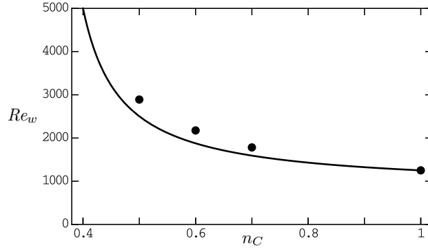
FIGURE 16. \circ , asymptotic values of the critical wall-viscosity Reynolds number Re_{wcpl}(n_C) for n_C = 0.5, 0.6, 0.7 together with the Newtonian value Re_{wcpl}(1) = Re_{cN} ; continuous curve, formula (5.18).
