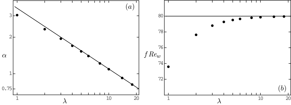
FIGURE 4. For n_C = 0.5 . (a): \circ , parameter \alpha defining the pressure gradient in the base flows, see (3.2). (b): \circ , scaled friction factor of the base flows. Full lines, power-law fluid case.
