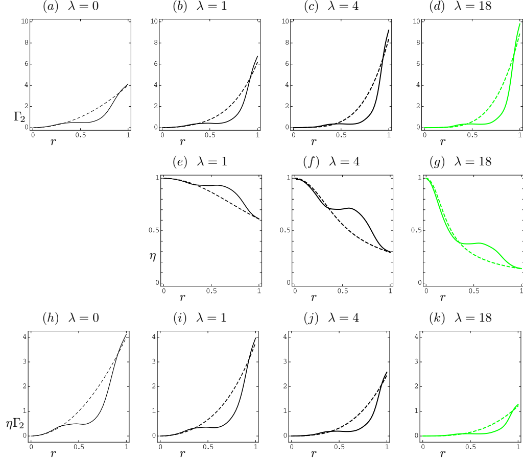
FIGURE 14. (Colour online) For n_C = 0.5 and various values of \lambda as indicated. (a – d) : full line, invariant \Gamma_2 averaged over \theta and z of the critical wave; dashed line, invariant \Gamma_2 of the laminar flow, already displayed in figure 2(b). (e – g) : full line, viscosity \eta averaged over \theta and z of the critical wave; dashed line, viscosity \eta of the laminar flow, already displayed in figure 2(c). (h – k) : full line, product \eta\Gamma_2 averaged over \theta and z of the critical wave; dashed line, same product in the laminar flow.
