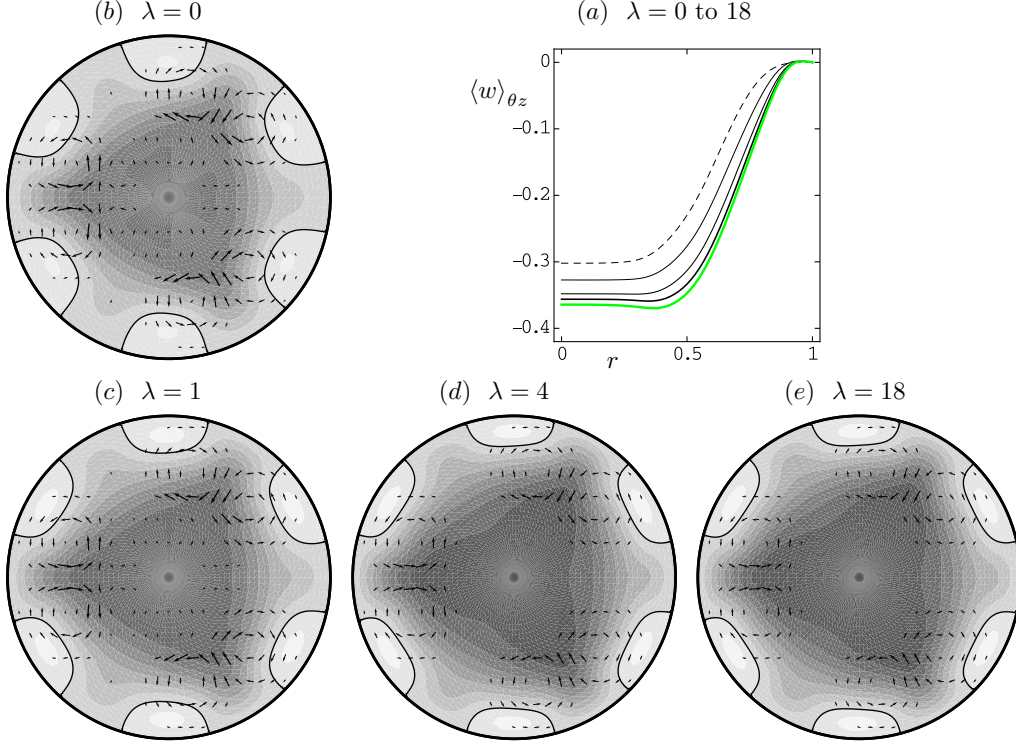
FIGURE 11. (Colour online) For n_C = 0.5 . (a): Axial velocity w = v_z - W_b averaged over \theta and z of the critical wave for different values of \lambda as in figure 10(a). (b – e): Axial average of the velocity field of the critical wave for various values of \lambda as indicated. The gray levels show the values of \langle w \rangle_z with 9 regularly spaced contours w = -0.35 (dark) to +0.05 (light). The contour w = 0 is shown with a black continuous line to evidence the fast streaks. The arrows show the transverse velocity vectors as in figures 10(b – e).
