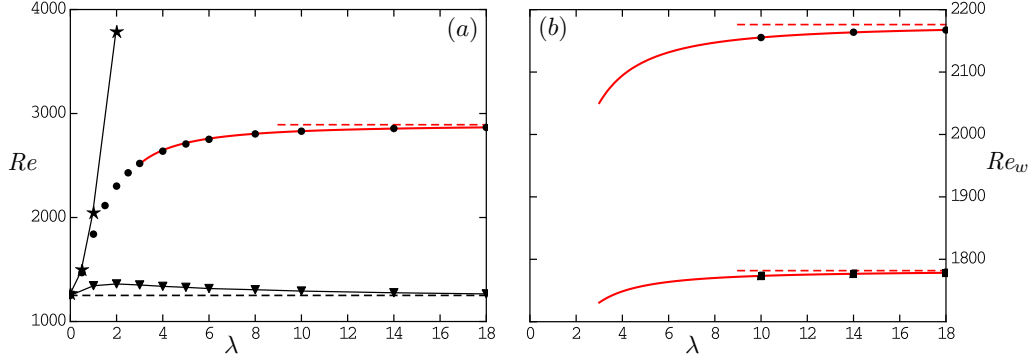
FIGURE 15. (Colour online) (a): for n_C = 0.5 . \star , onset wall-viscosity Reynolds number Re_w(q_{cN}; n_C, \lambda) found by RPN2010; \circ , after optimisation of the wavenumber q , critical wall-viscosity Reynolds number Re_{wc}(n_C, \lambda) ; \nabla , critical mean-viscosity Reynolds number Re_{mc}(n_C, \lambda) ; gray (red online) curve, fit (5.15); upper dashed line, asymptotic value (5.16); lower dashed line, critical value of the Newtonian case Re_{cN} (1.2). (b): \circ , for n_C = 0.6 , \square , for n_C = 0.7 , critical wall-viscosity Reynolds number Re_{wc}(n_C, \lambda) ; gray (red online) curves, fits (5.15), dashed lines, asymptotic values (5.19).
