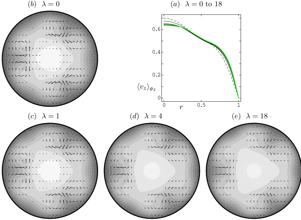
FIGURE 10. (Colour online) For n_C = 0.5 . (a): Total axial velocity v_z averaged over \theta and z of the critical wave for different values of \lambda as in figure 2: the curves ordered by decreasing centerline velocities correspond to \lambda = 0, 1, 2, 4, 18 . (b – e): Axial average of the velocity field of the critical wave for various values of \lambda as indicated. The gray levels show the values of \langle v_z \rangle_z with 9 regularly spaced contours v_z = 0.07 (dark) to 0.63 (light). The arrows show on a cartesian grid the transverse velocity vectors \mathbf{v}_\perp = \langle u \rangle_z \mathbf{e}_r + \langle v \rangle_z \mathbf{e}_\theta whose norm \|\mathbf{v}_\perp\| \geq 0.003 . The scale of the arrows is the same on all graphs: \max \|\mathbf{v}_\perp\| decreases as \lambda increases.
