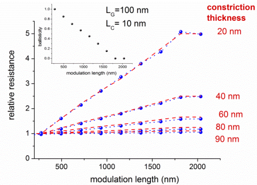
Figure 4b As in Figure 3a, for the relative resistance. The inset shows the fitting parameter \chi versus the modulation length.
