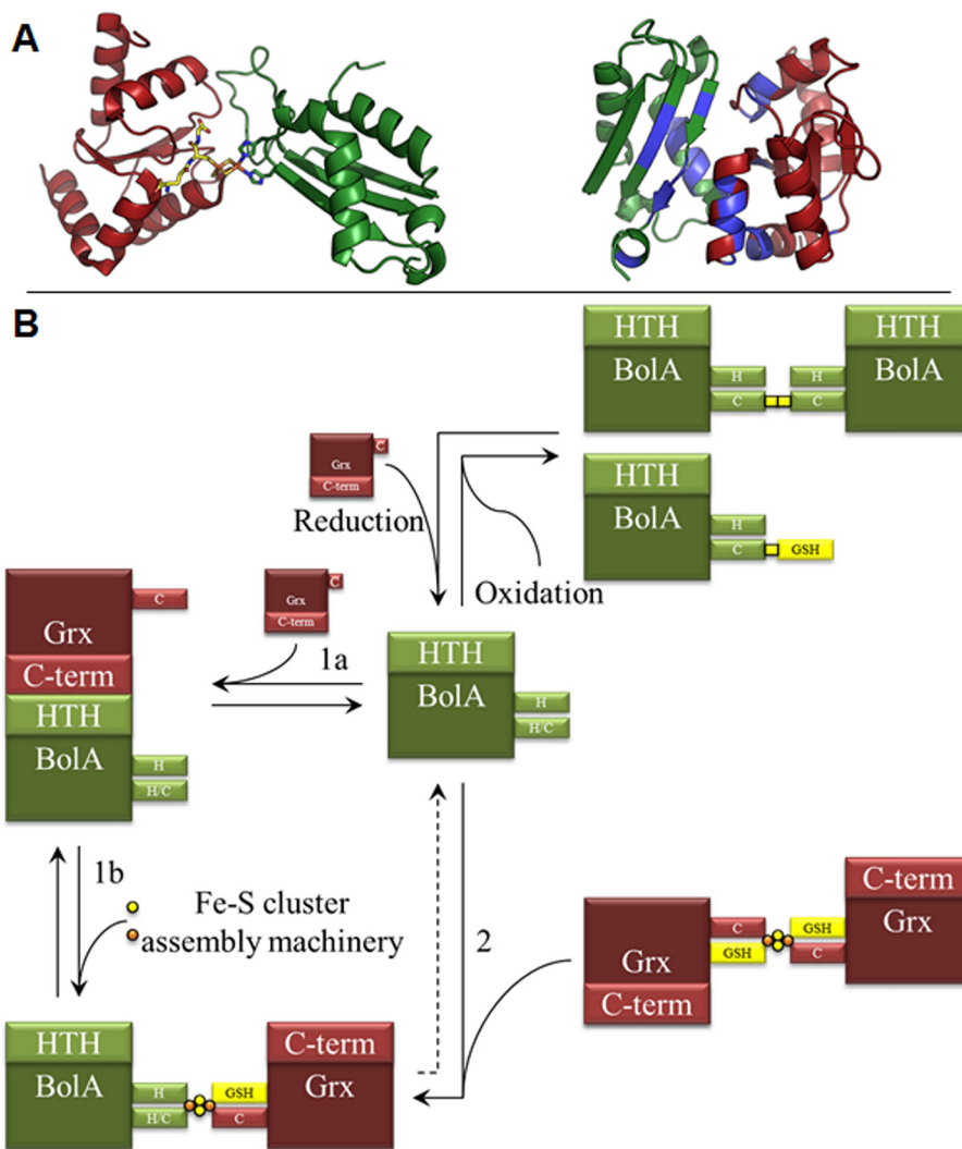
FIGURE 6. Formation of BolA-Grx complexes. A , comparison of AtGrxS14-BolA apo- and holo-heterodimers. The [2Fe-2S]-bridged AtGrxS14-BolA1 holo-heterodimer model was built from the structures of individual proteins. The model of AtGrxS14-BolA2 apo-heterodimer was obtained by NMR-based docking from residues (colored in blue ) presenting high chemical shift variations upon partner addition. Grxs are colored in green , BolA are in red , and glutathione is in yellow . B , recapitulative scheme showing the formation of BolA-BolA and Grx-BolA complexes. From the current literature, there are two pathways to form Grx-BolA holo-heterodimers. Grx-BolA apo-heterodimers can accept a [2Fe-2S] cluster from IscAs or possibly other Fe-S assembly components ( pathway 1 ) (50). Alternatively BolA can displace a Grx monomer from holo-homodimeric Grxs as shown for the ScGrx3-Fra2 couple ( pathway 2 ) (7). In principle, the reactions are reversible, and monomeric BolAs or Grx-BolA apo-heterodimers could be reformed by disruption (7) of the Grx-BolA holo-heterodimer Fe-S cluster or its transfer to an acceptor. Due to the presence of a cysteine residue, BolA_Cs can form disulfide bridges either as covalent dimers or as glutathionylated forms, both forms being reversibly reduced by Grxs (10). The physiological relevance of each form has not been always elucidated, but interconversion can affect all assumed functions of both proteins (DNA binding, iron-sensing, or Fe-S cluster maturation).
