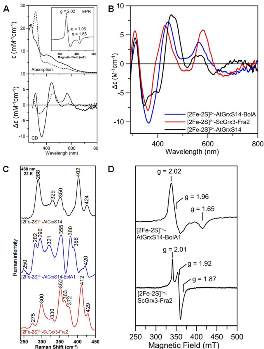
FIGURE 5. Spectroscopic studies of AtGrxS14-BolA1 holo-heterodimers. A , UV-visible absorption and CD spectra of oxidized ( solid line ) and dithionite-reduced ( broken line ) reconstituted AtGrxS14-BolA1 complex. \epsilon and \Delta\epsilon values are expressed per AtGrxS14-BolA1 heterodimer, and the intense band at 314 nm in the reduced absorption spectrum arises from excess dithionite. The inset shows the X-band EPR spectrum of the dithionite-reduced sample recorded at 10 K and 9.581 GHz, with a microwave power of 5 milliwatts and a modulation amplitude of 0.65 millitesla. B , comparison of the CD spectra of the [2\text{Fe-2S}]^{2+} centers in the AtGrxS14-BolA1 and ScGrx3-Fra2 heterodimers and the AtGrxS14 homodimer. \Delta\epsilon values are expressed per [2\text{Fe-2S}]^{2+} cluster. C , comparison of the resonance Raman spectra of the [2\text{Fe-2S}]^{2+} centers in the AtGrxS14-BolA1 and ScGrx3-Fra2 heterodimers and the AtGrxS14 homodimer. Spectra were recorded using 488-nm laser excitation. Samples were \sim 2 mm in the [2\text{Fe-2S}] cluster and were in the form of a frozen droplet at 17–22 K. Each spectrum is the sum of 100 scans, with each scan involving photon counting for 1 s at 0.5\text{ cm}^{-1} increments with 6\text{ cm}^{-1} spectral resolution. Bands due to lattice modes of ice have been subtracted from all spectra. D , comparison of the X-band EPR spectra of the dithionite-reduced [2\text{Fe-2S}]^{1+} centers in the AtGrxS14-BolA1 and ScGrx3-Fra2 heterodimers. EPR conditions: microwave frequency, 9.581 GHz; modulation amplitude, 0.65 millitesla; microwave power, 5 milliwatts; temperature, 10 K. Spin quantification of both EPR signals indicates 1.0 \pm 0.1 spins per [2\text{Fe-2S}] cluster.
