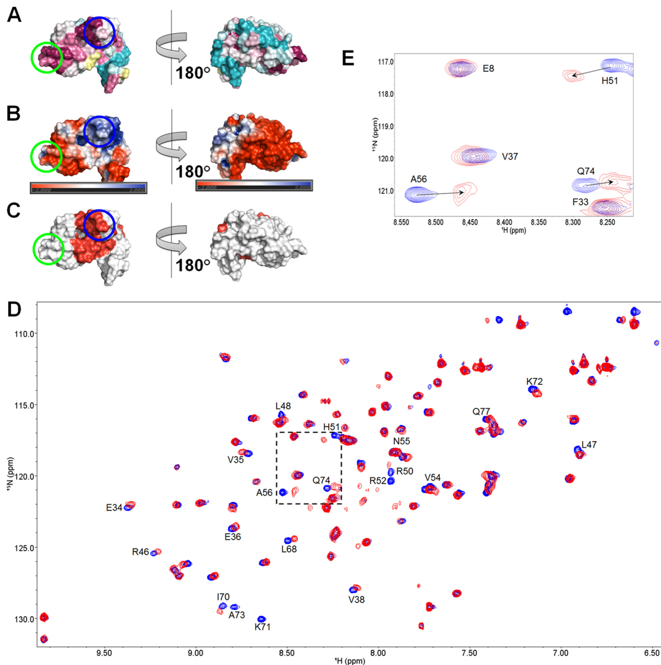
FIGURE 2. Interaction of AtBola2 with AtGrxS14. A, the left panel displays the conserved face of BolAs, and the right panel displays the variable face of BolAs. Residue conservation ranges from 0% (cyan) to 100% (purple). RHR signature (blue circle) and putative ligands of the [2Fe-2S] cluster (green circle) are also highlighted on AtBola2 surface. B, electrostatic potential of AtBola2 generated by APBS (57) and showing negative charges in red and positive charges in blue. C, mapping of the residues of AtBola2 (red) involved in the interaction with AtGrxS14, as shown by NMR. D, overlay of ^1\text{H} , ^{15}\text{N} HSQC spectrum of AtBola2 (blue) and ^1\text{H} , ^{15}\text{N} HSQC spectrum of AtGrxS14-Bola2 at a 1:1 ratio (red). The assigned peaks are indicated with the residue number and one-letter code. E, zoom of the area delimited by dashed lines in D. The arrows indicate the direction in which the amide peak shifts upon the addition of AtGrxS14.
