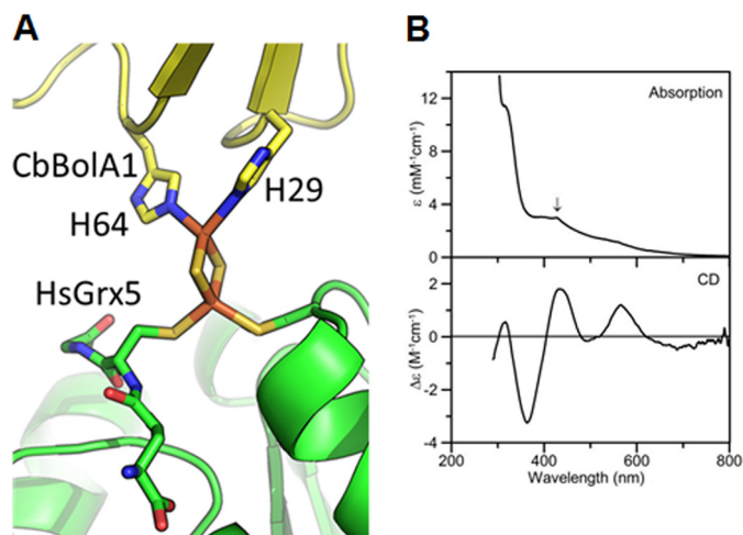
FIGURE 4. Glutaredoxin-Bola H holo-heterodimer. A, model of the Grx-Bola holo-heterodimer with Rieske-type [2\text{Fe}-2\text{S}] coordination built using human Grx5 (PDB entry 2WUL) (58) and C. burnetii Bola, which coordinates a cobalt atom via His-29 and His-64 (PDB entry 3TR3). These residues are ideally positioned to coordinate an iron atom of a [2\text{Fe}-2\text{S}] cluster instead of cobalt, and they were used to orientate the Bola domain in the heterodimeric model. B, UV-visible absorption and CD spectra of AtGrxS14-Bola1 heterodimers. \epsilon and \Delta\epsilon values are expressed per AtGrxS14-Bola1 heterodimer, and the arrow indicates the Soret band from a trace heme impurity. AU, arbitrary units.
